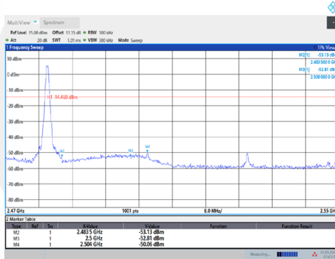
DH5_Ant1_High_2480
