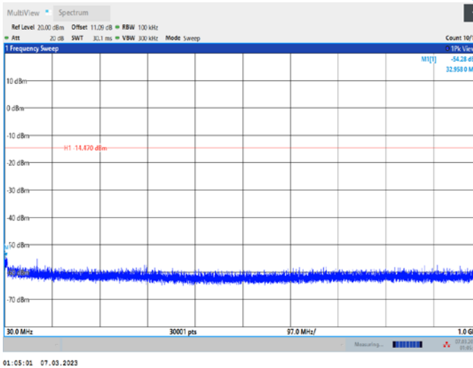
DH5_Ant1_2441_30~1000
