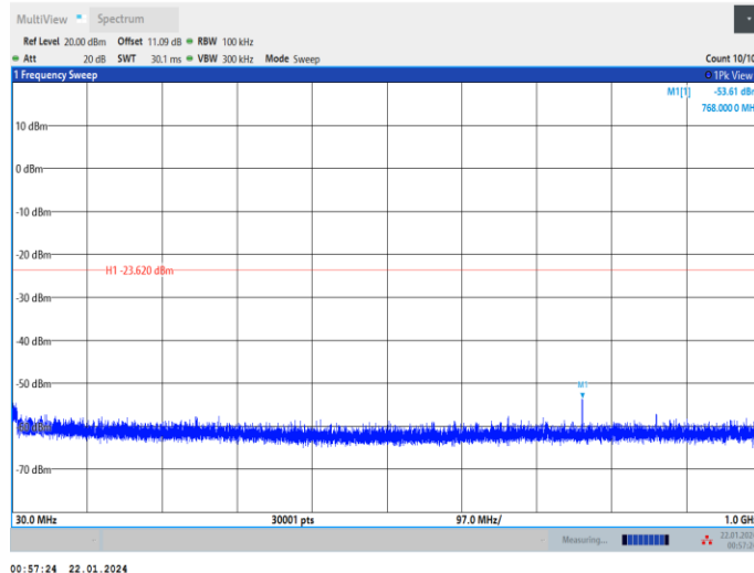
DH5_Ant1_2441_30~1000
