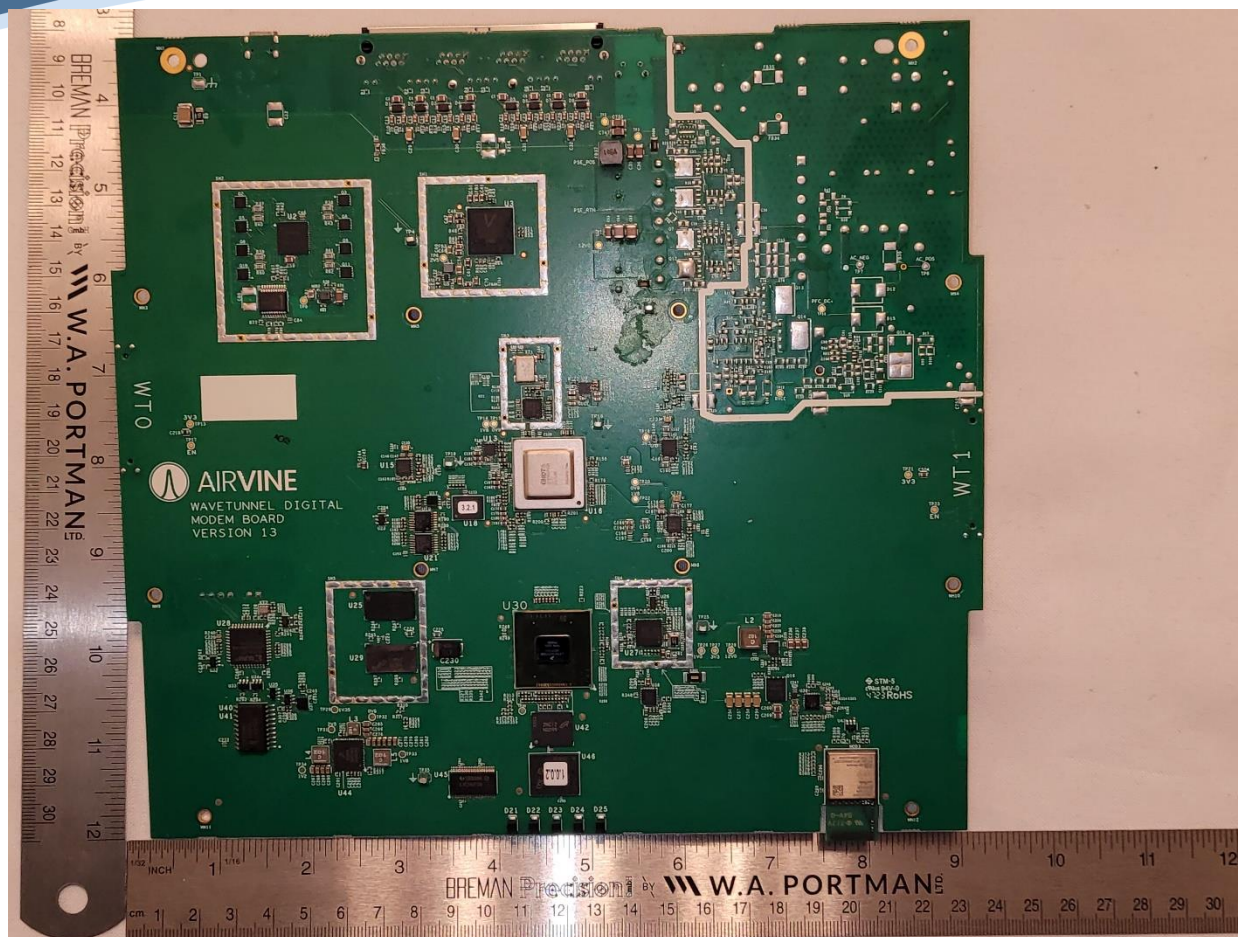
Digital Board Top
