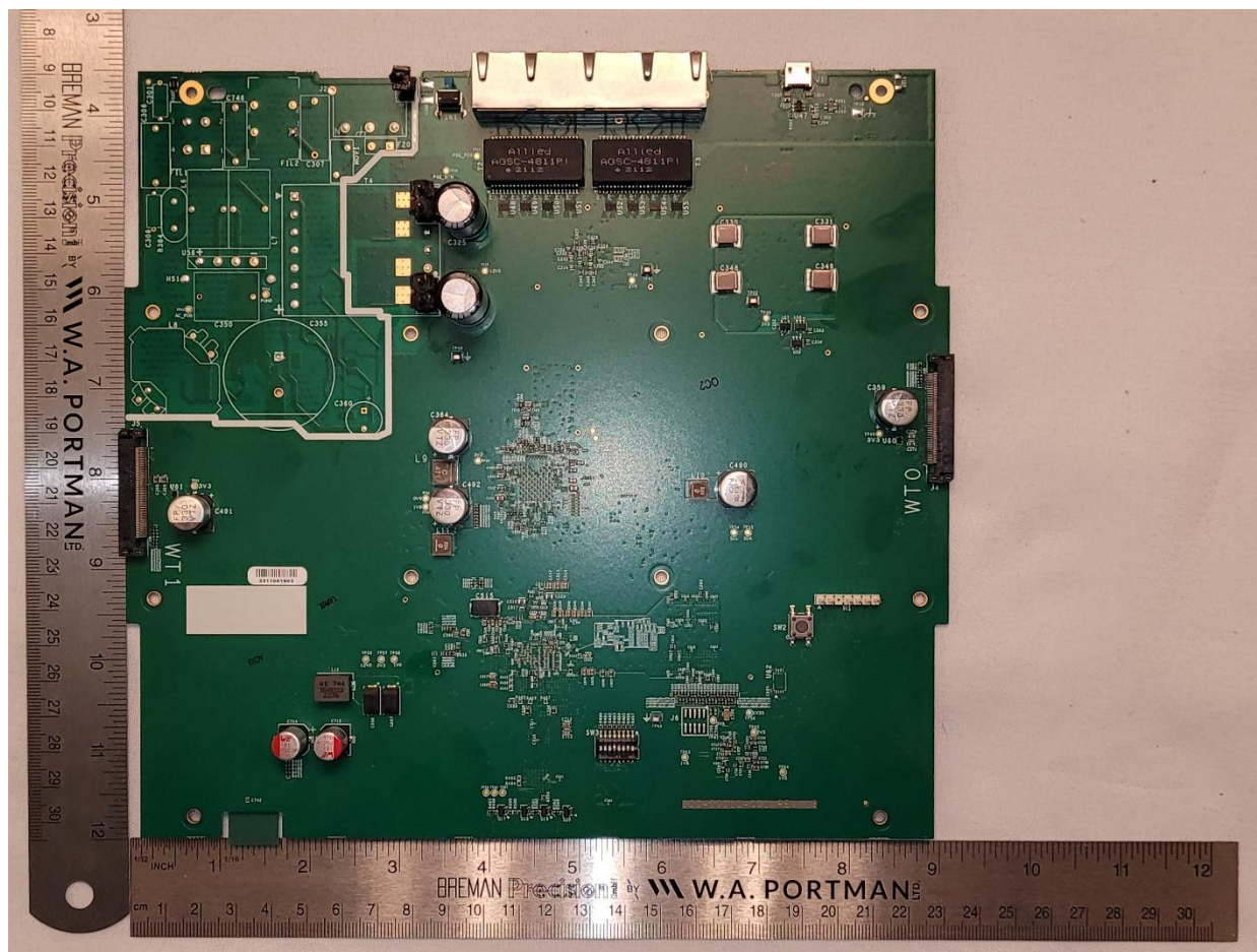
Digital Board Bottom
