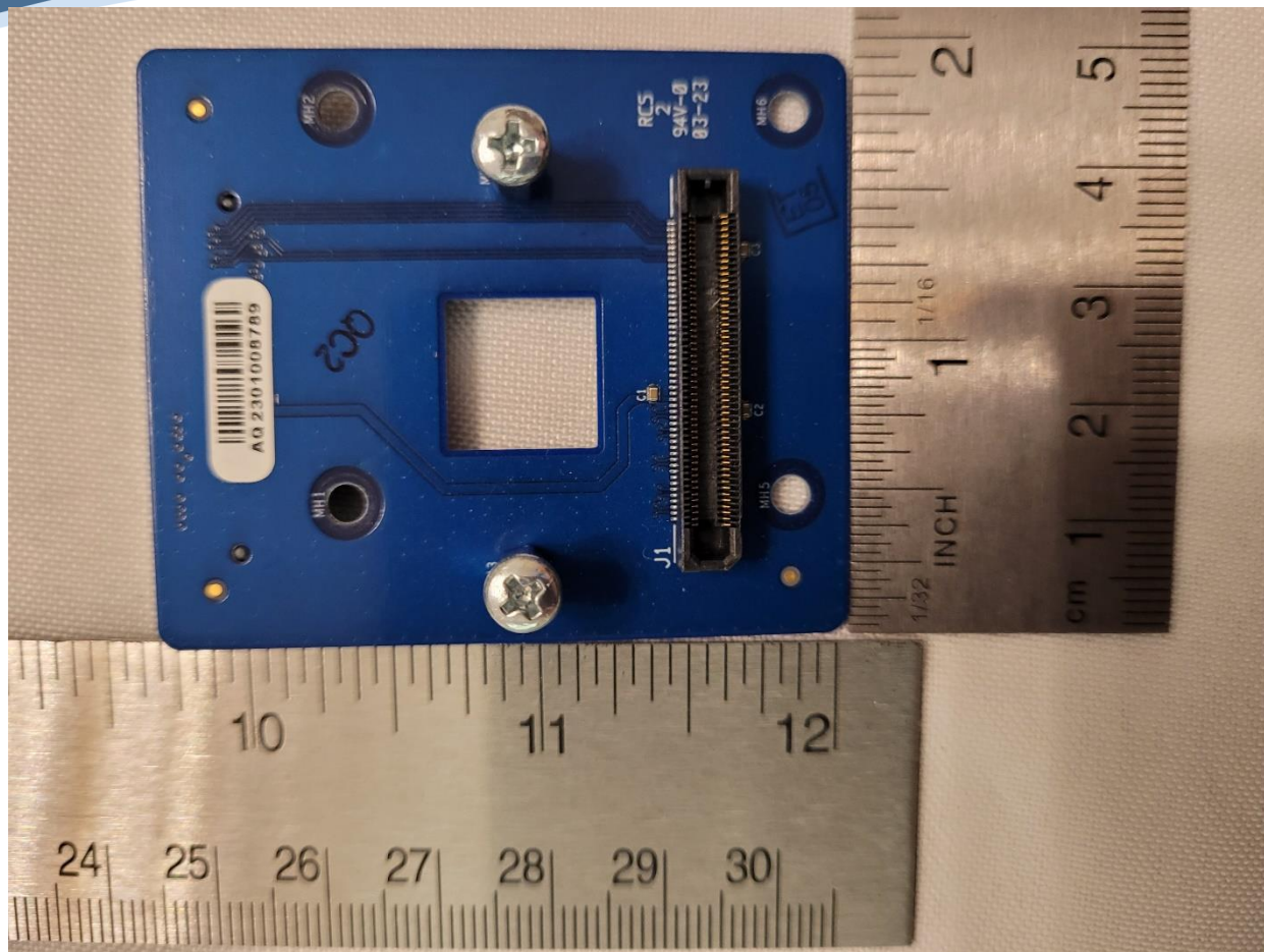
Interface Board Top
