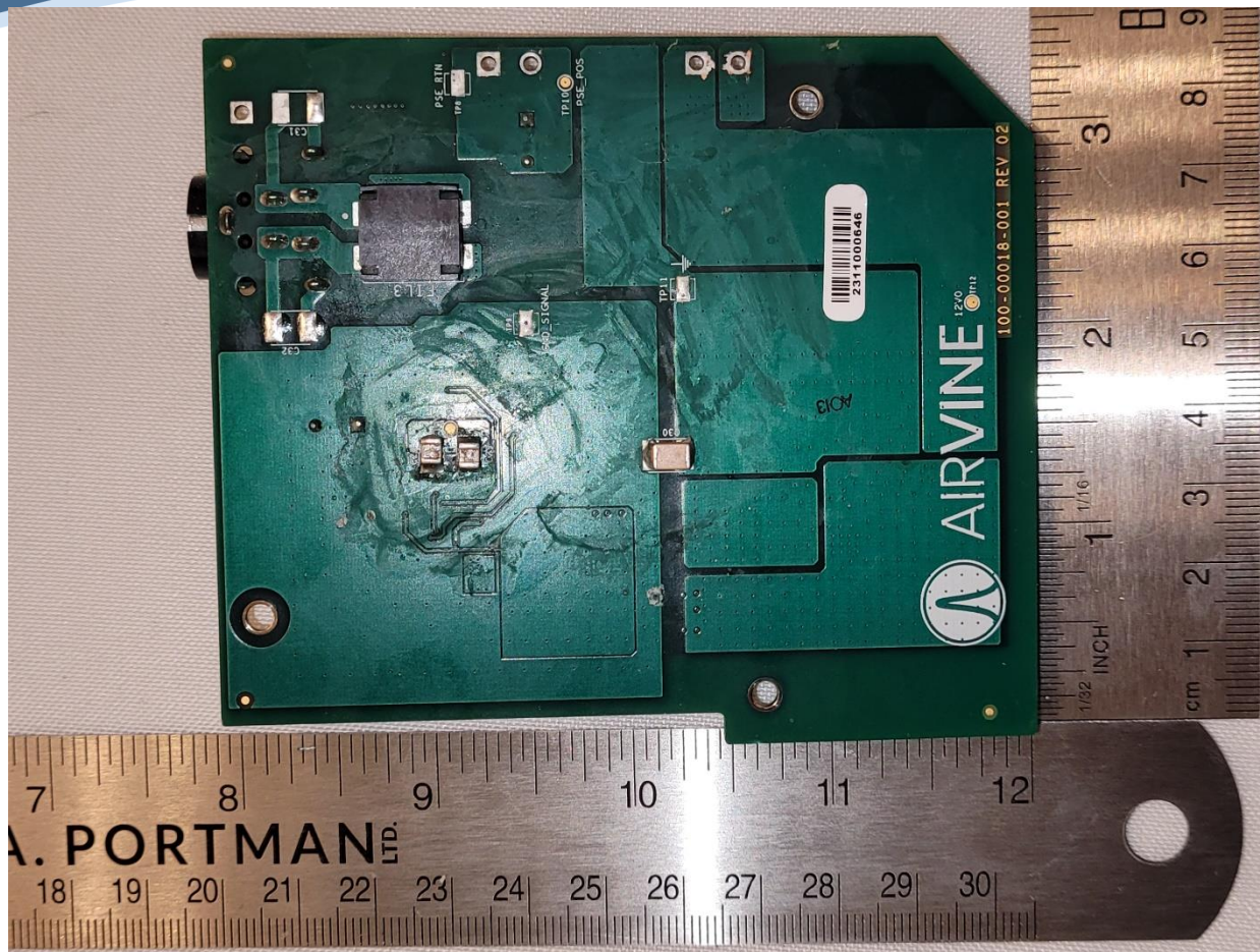
Power Board Top
