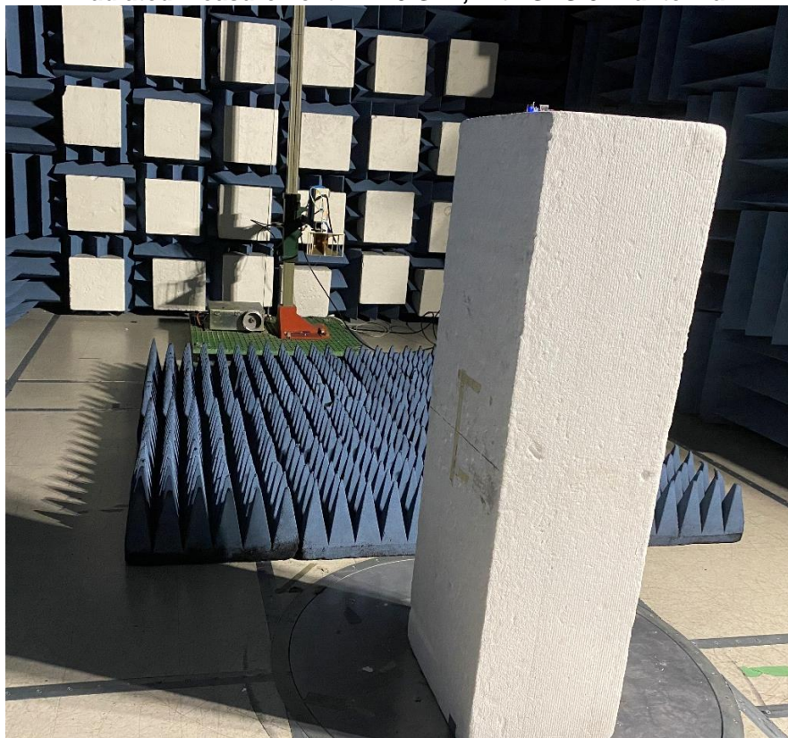
Radiated measurement 1 – 18 GHz, with SAS-571 antenna
