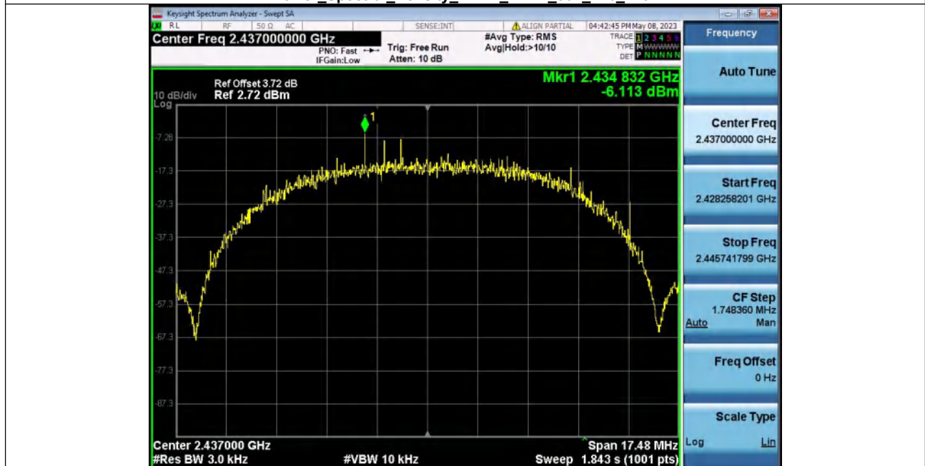
Power_Spectral_Density_NVNT_ANT1_802_11b_2437
