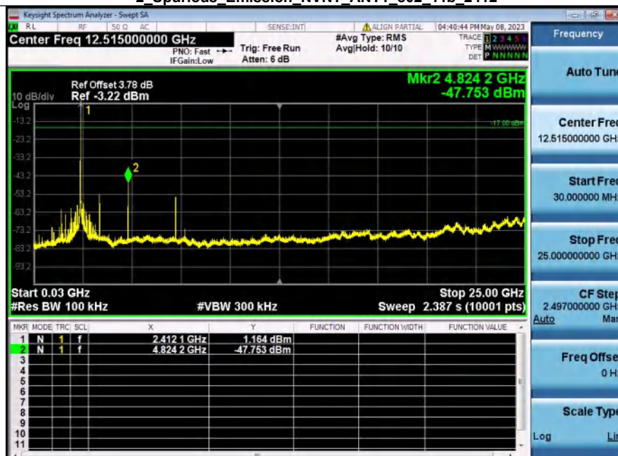
2 Spurious_Emission_NVNT_ANT1_802_11b_2412
