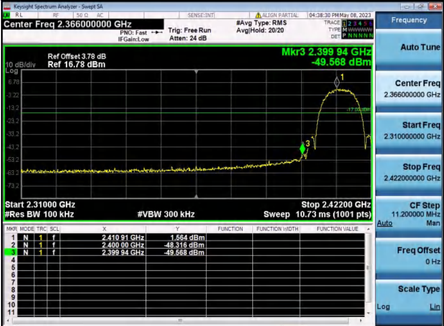
2 Bandedge NVNT_ANT1_802_11b_2412
