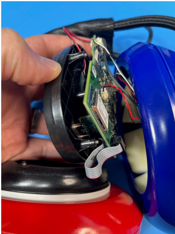
Charging port connection (View 1)
