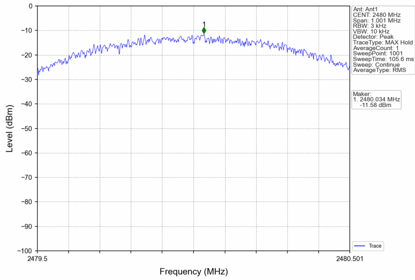
1M_HCH_2480MHz_Ant1_NTNV
