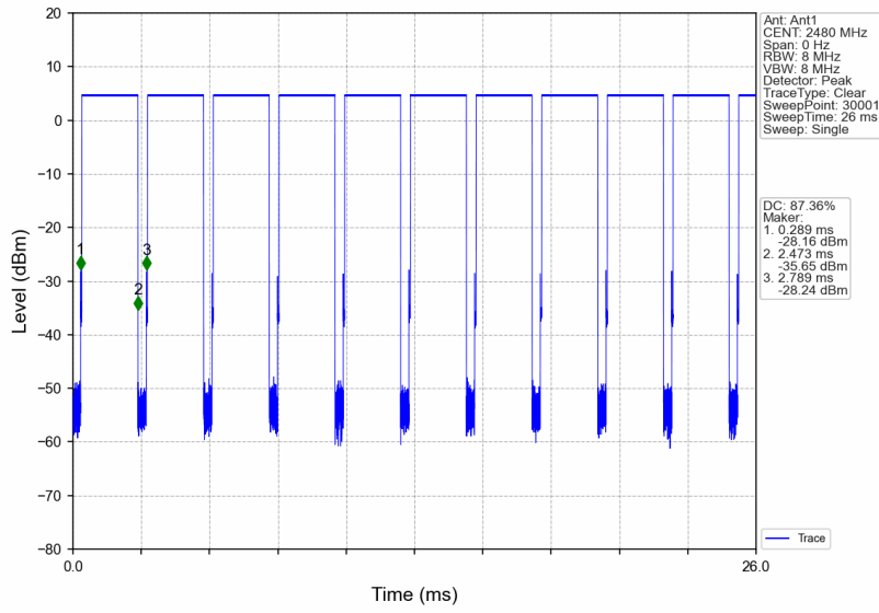
1M_HCH_2480MHz_Ant1_NTNV
