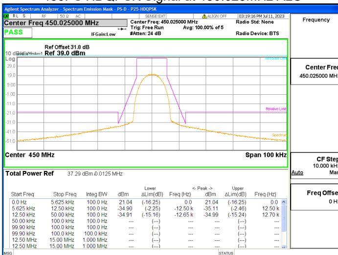
450PS HDQPSK Signal at 450.025MHz ALC
