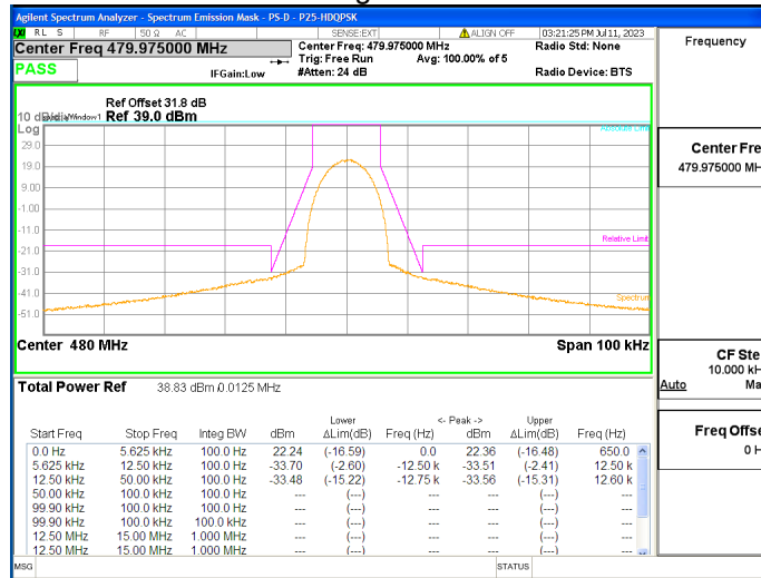
450PS HDQPSK Signal at 479.975MHz ALC
