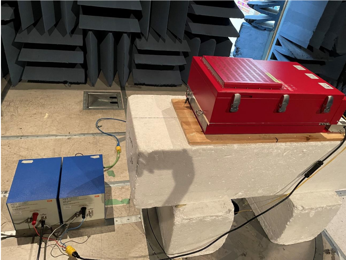
Figure 4: Conducted Emissions Test Setup at AC Main
