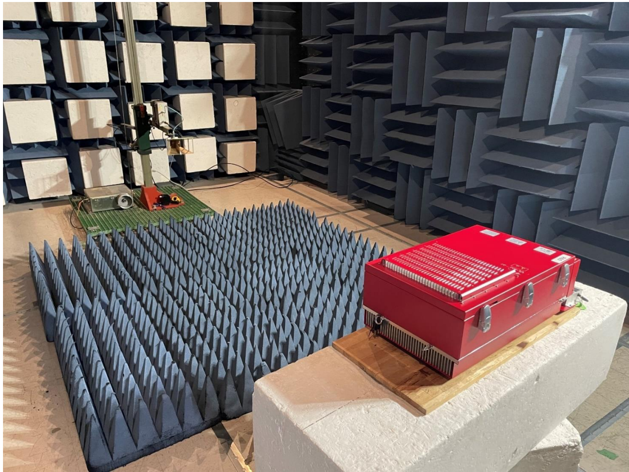
Figure 3: Radiated Emissions (Above 1GHz) Test Setup
