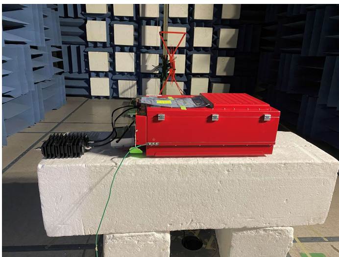
Figure 2: Radiated Emissions (Below 1GHz) Emissions Test Setup
