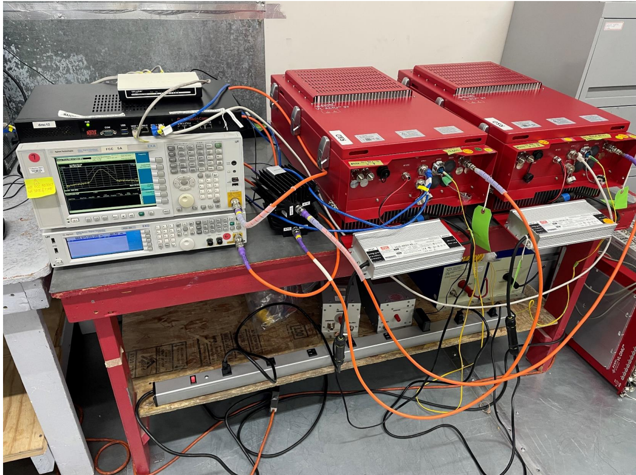
Figure 1: RF Conductive Emissions Test Setup
