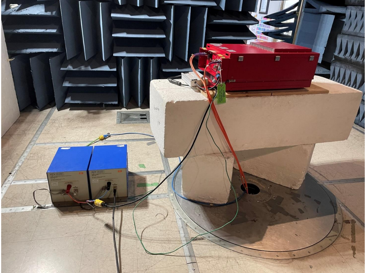
Figure 4: Conducted Emissions Test Setup at AC Main
