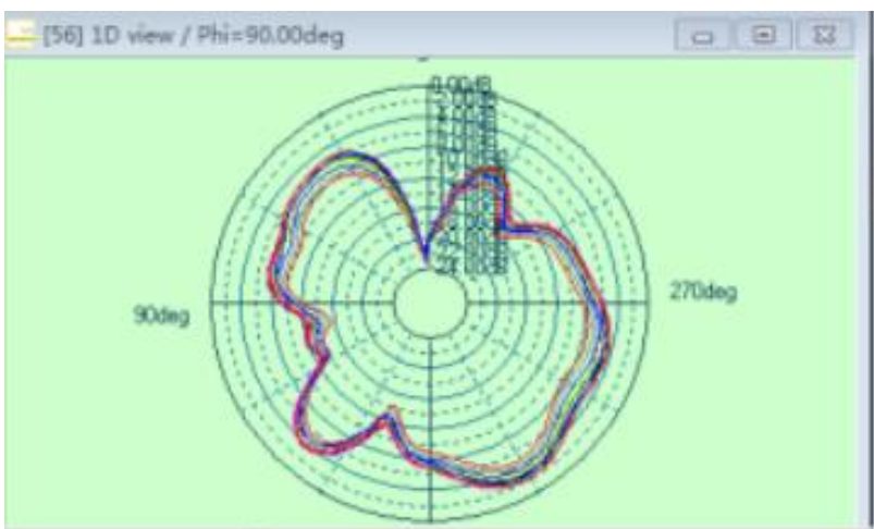
R-Radiation pattern: Phi=90°
