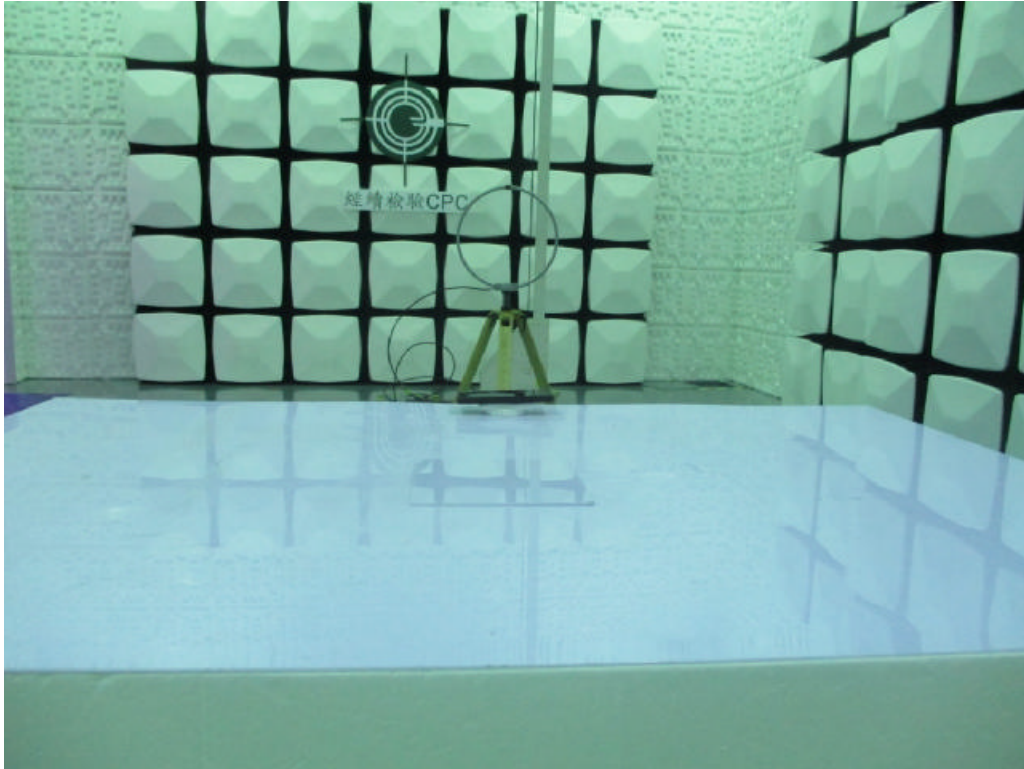
Setup Photo FCC ID: 2BA5S-CW80
