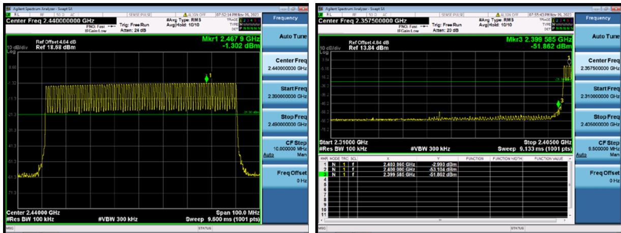
GFSK Hopping
