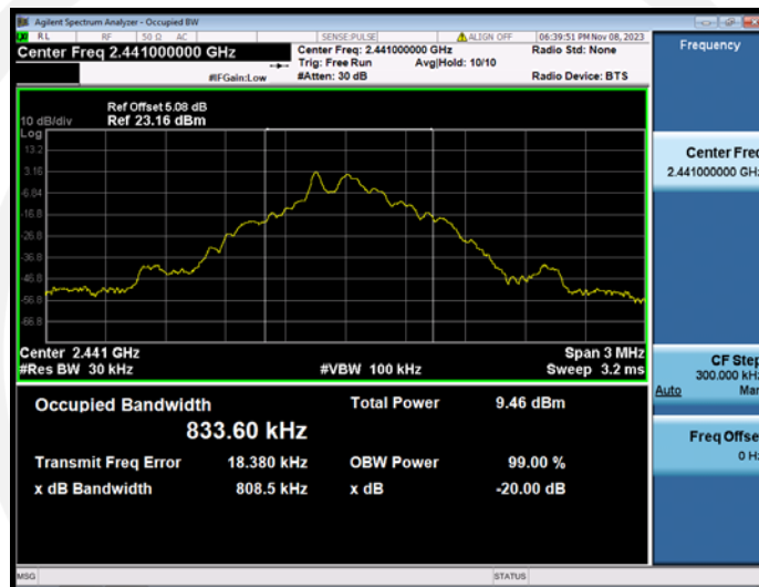
GFSK(1-DH1) 2441MHz
