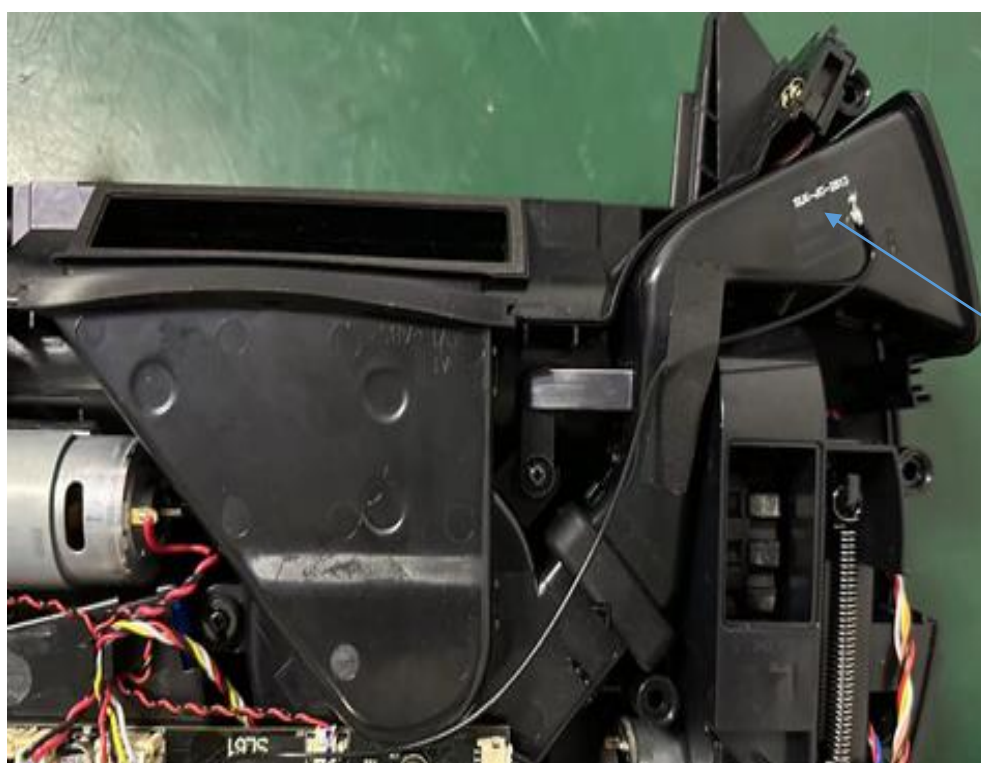
Wi-Fi antenna
