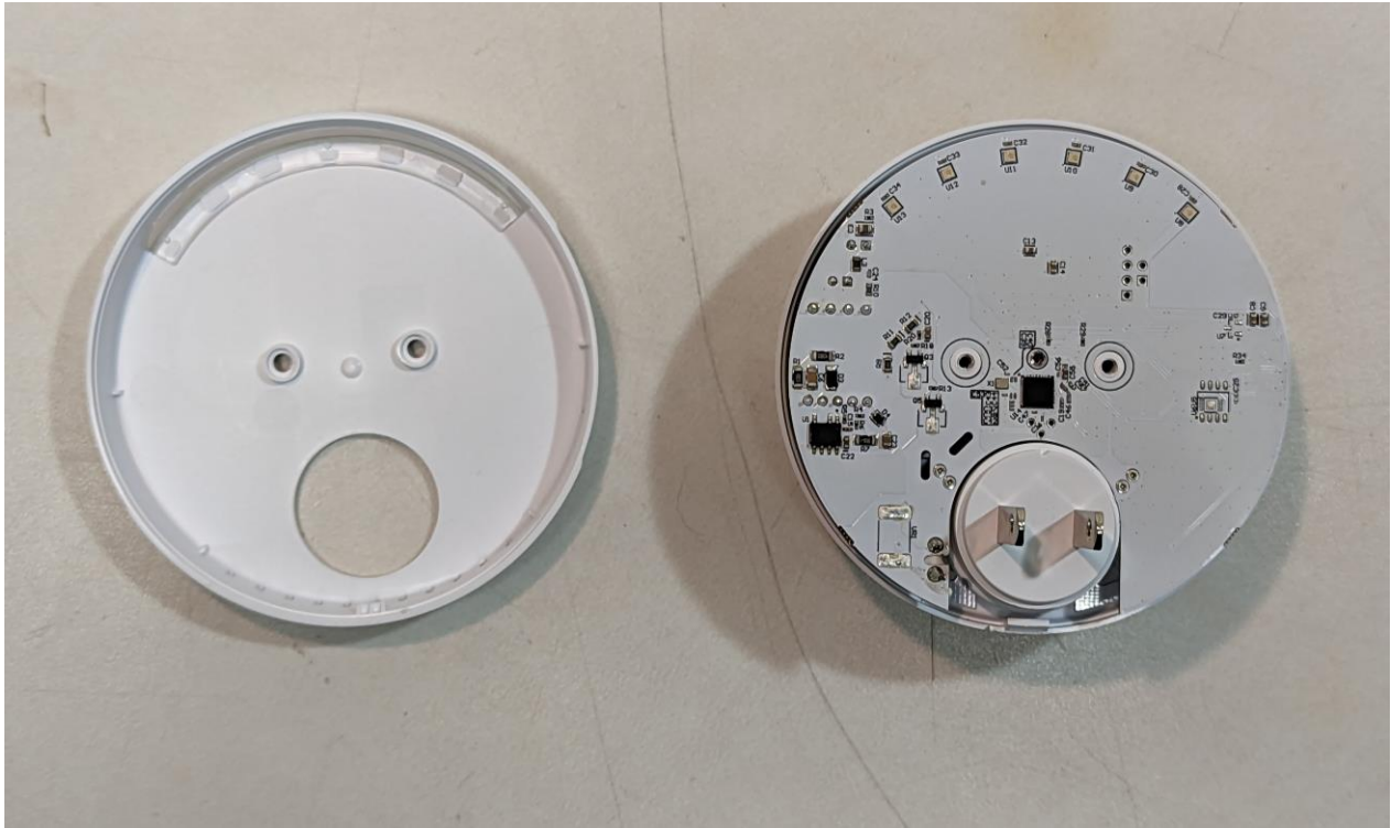
Photograph 4 – View of PCBA in the Housing
