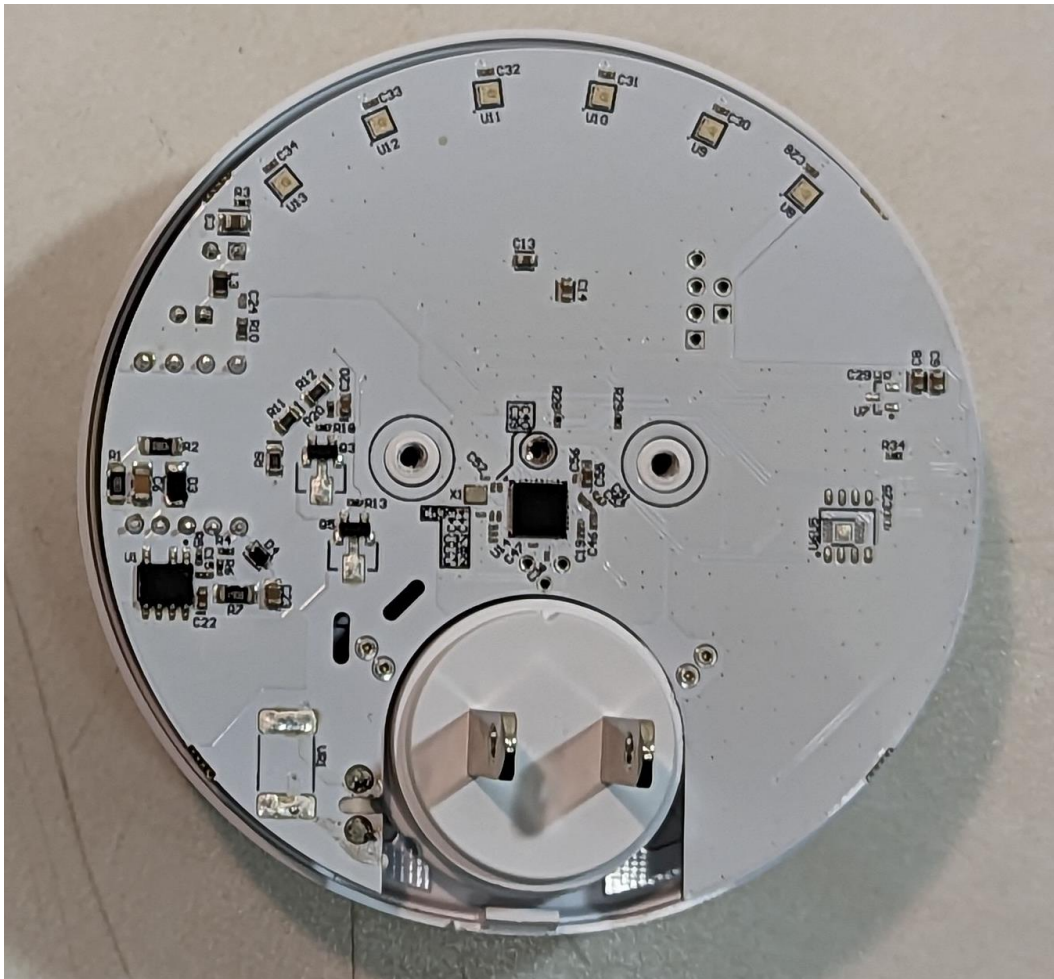
Photograph 2 – Back View of the PCBA
