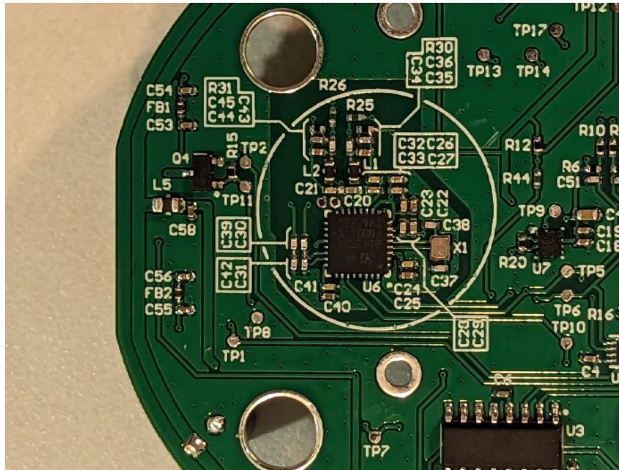
Photograph 3 – Close-up View of the RF Circuitry Under the Shield
