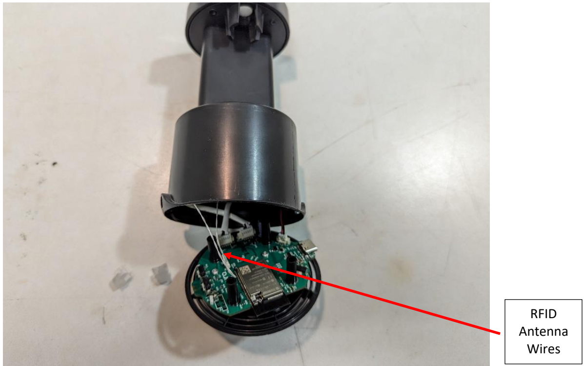
Photograph 5 – View of PCBA in the Housing with Cables and RFID Antenna Connection
