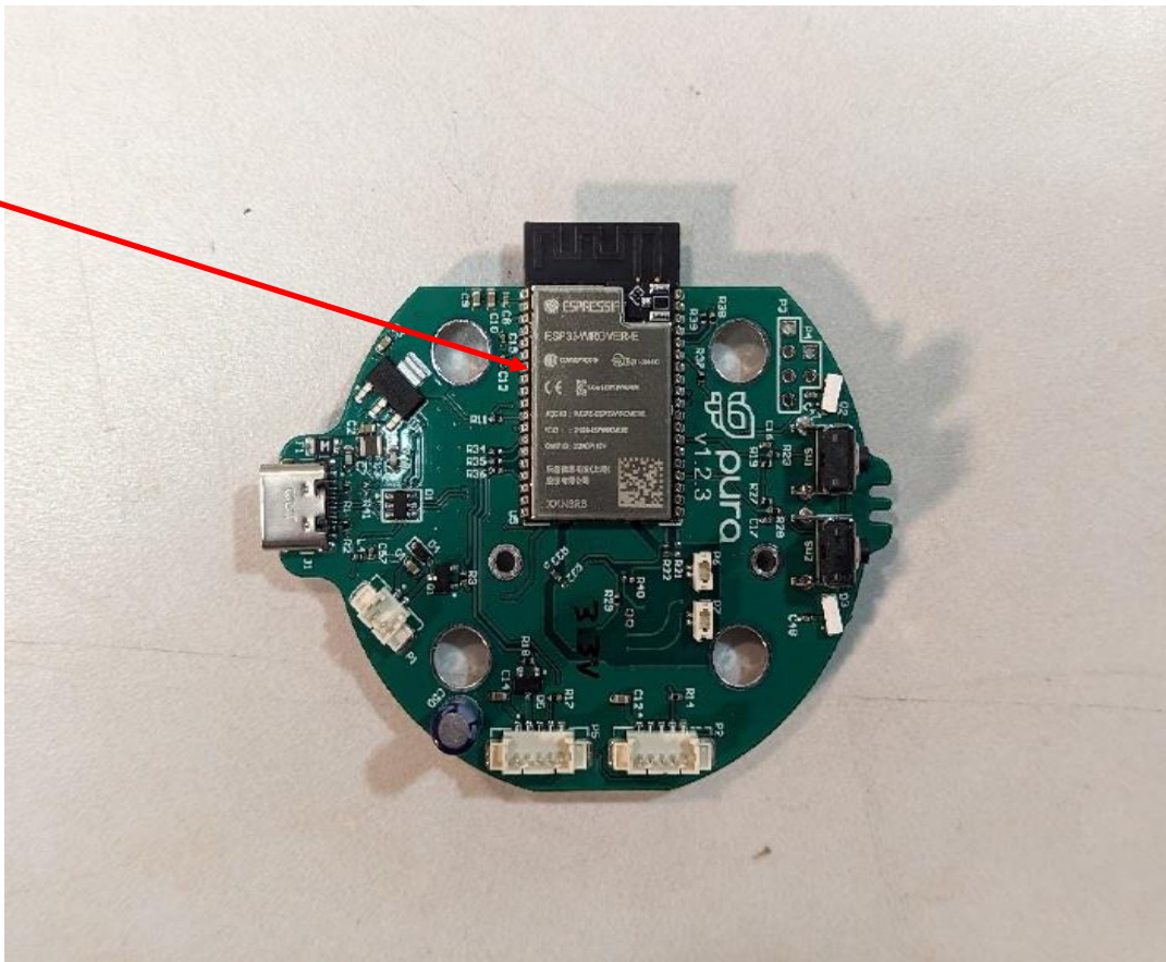
Photograph 1 – Front View of the PCBA
