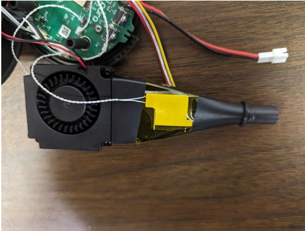
Photograph 6 – View of RFID Antenna Placement in Housing (One per side)
