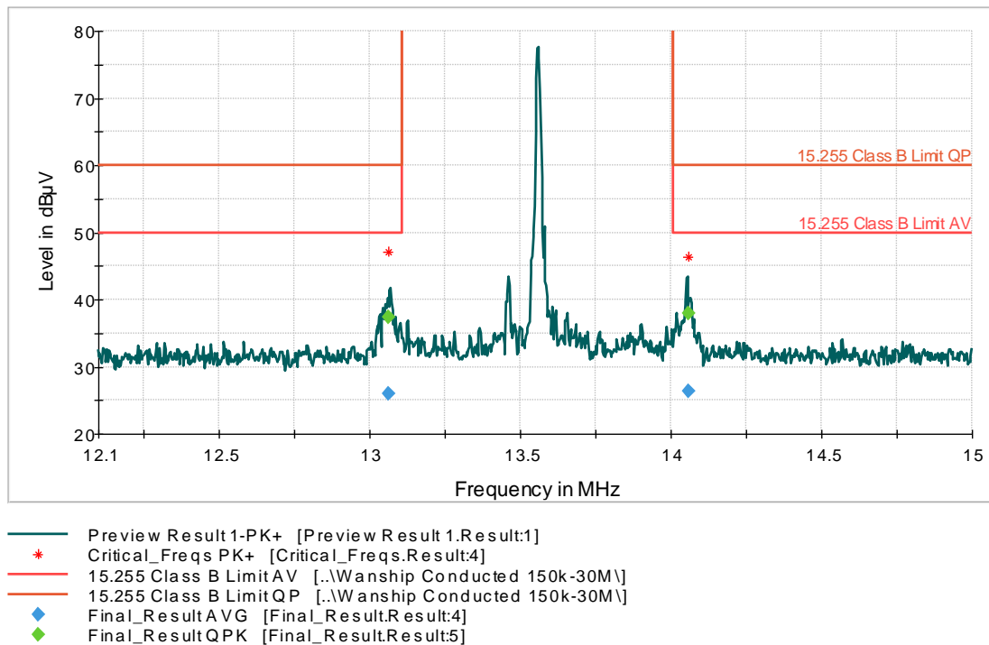
Graph 7: AC Mains Conducted Neutral Lead Fundamental Emission Band Edges with Tags – Antenna 2 Transmitting
