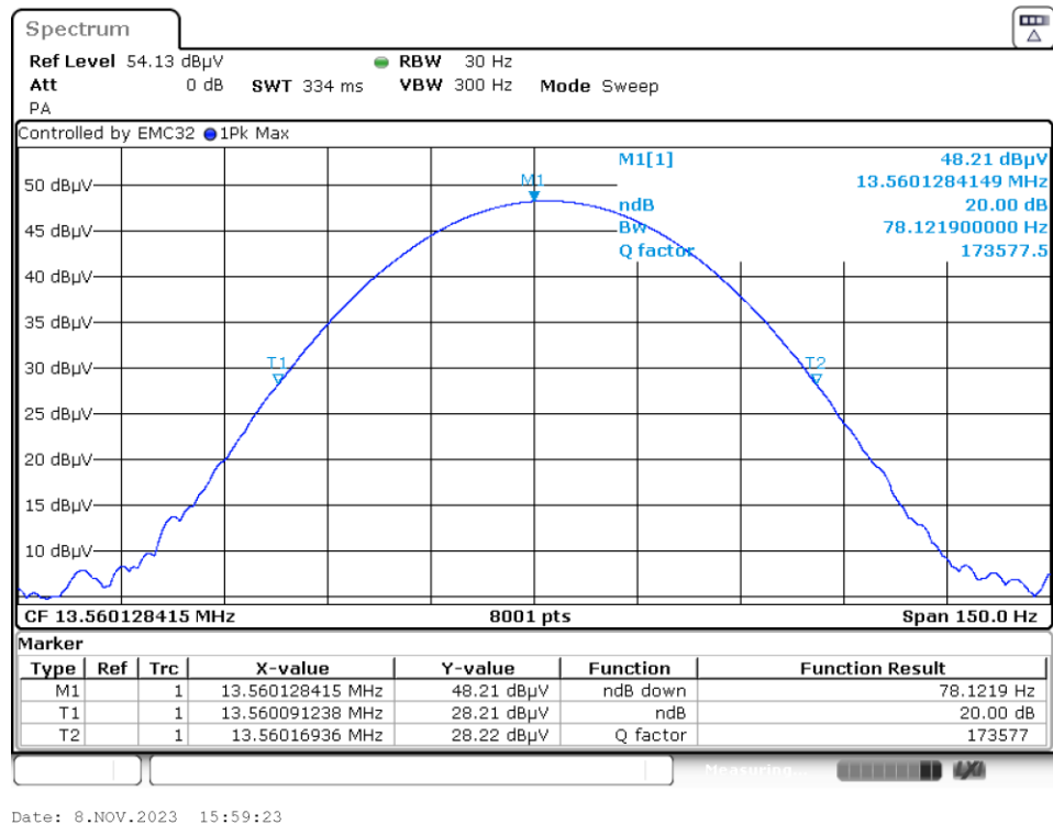
Graph 10: Worst-Case 20dB Bandwidth (Antenna 2 Transmitting)
