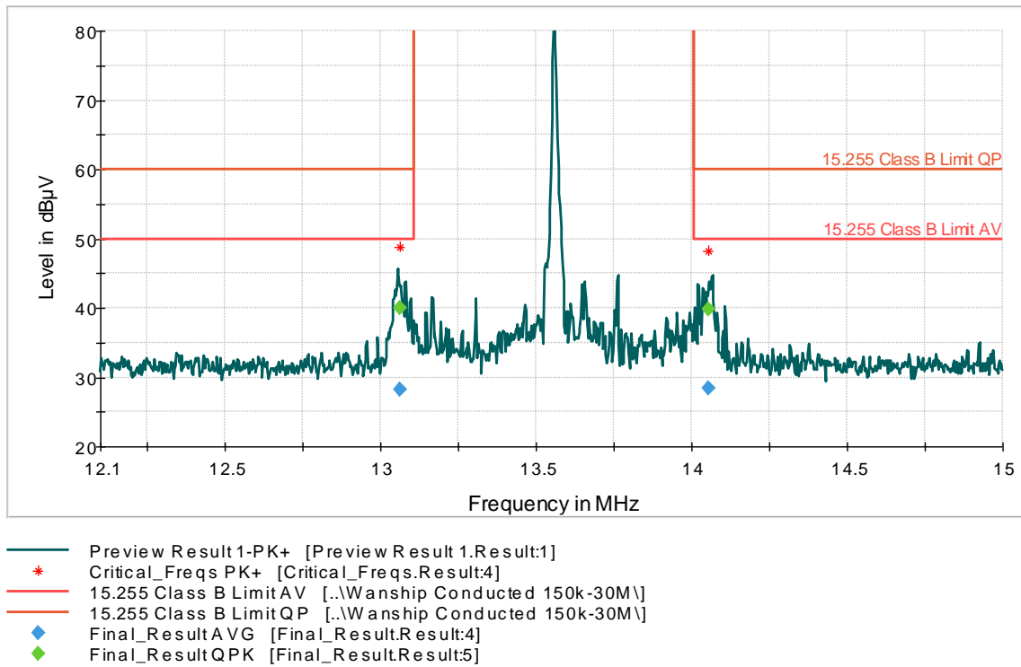
Graph 5: AC Mains Conducted Neutral Lead Fundamental Emission Band Edges with Tags – Antenna 1 Transmitting
