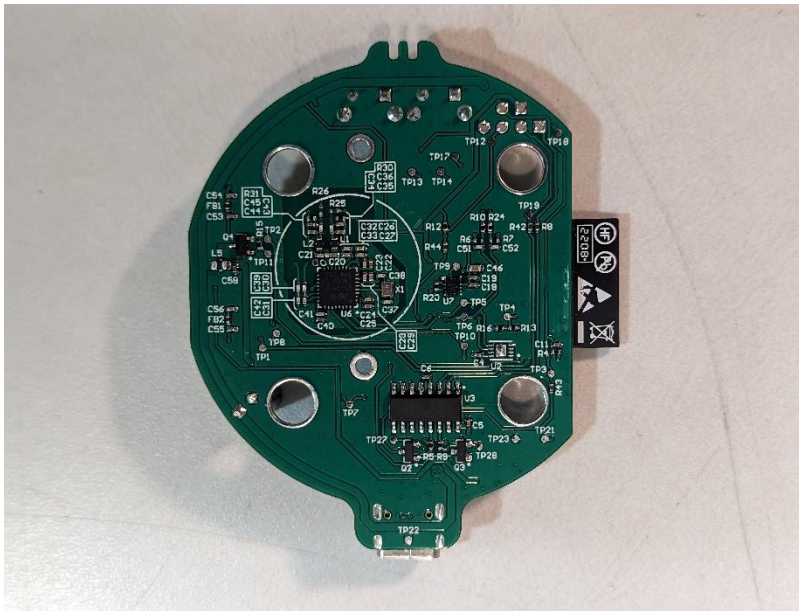
Photograph 23: Bottom View of PCB Removed from Enclosure with Ferrite Plate Removed
