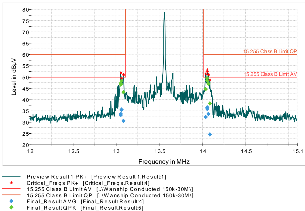
Graph 3: AC Mains Conducted Hot Lead Fundamental Emission Band Edges with Tags - Antenna 2 Transmitting
