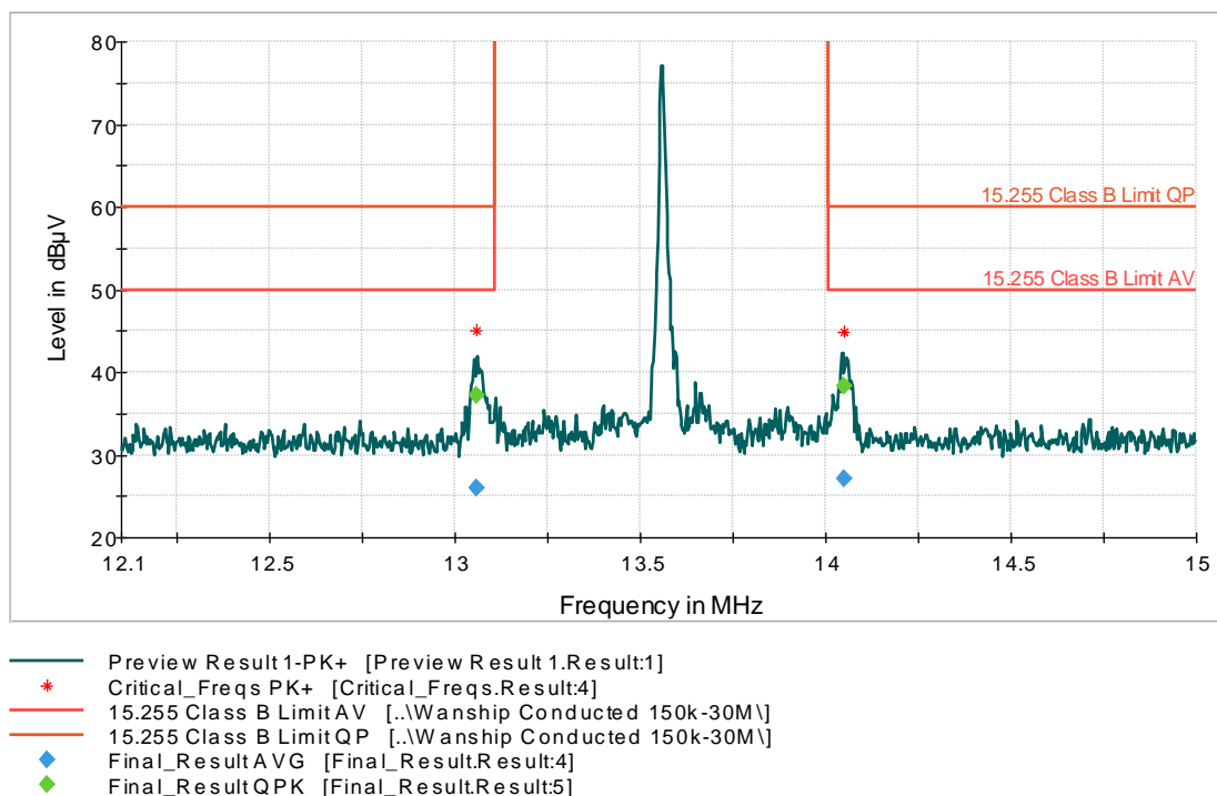
Graph 8: AC Mains Conducted Neutral Lead Fundamental Emission Band Edges without Tags – Antenna 2 Transmitting
