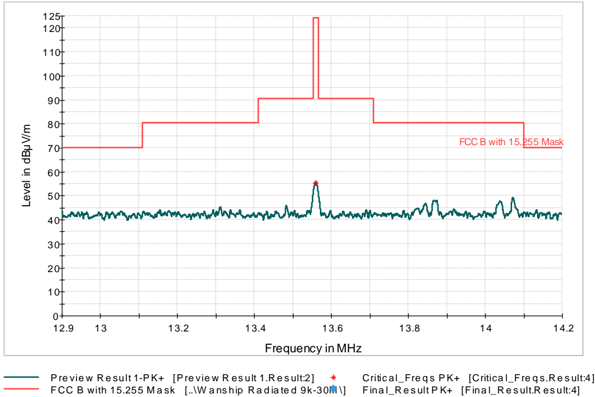
Graph 11: Antenna 1 with Tag
