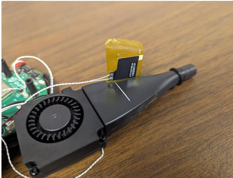
Photograph 26: View of NFC Antennas
