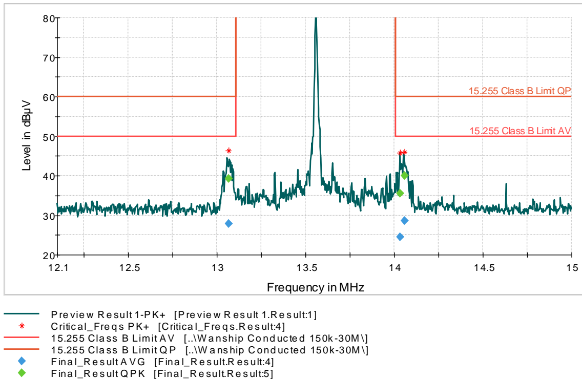
Graph 6: AC Mains Conducted Fundamental Neutral Lead Emission Band Edges without Tags – Antenna 1 Transmitting
