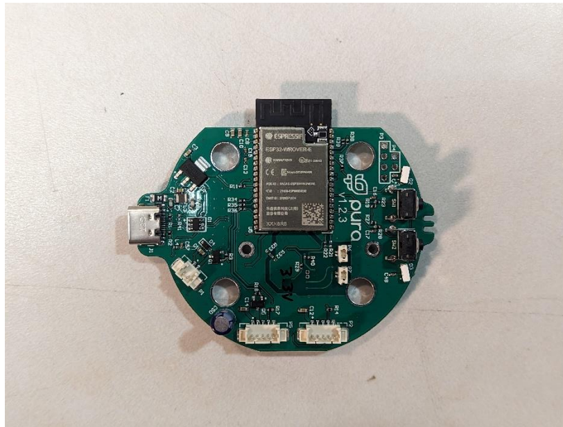
Photograph 17: Top View of PCB Removed from Enclosure
