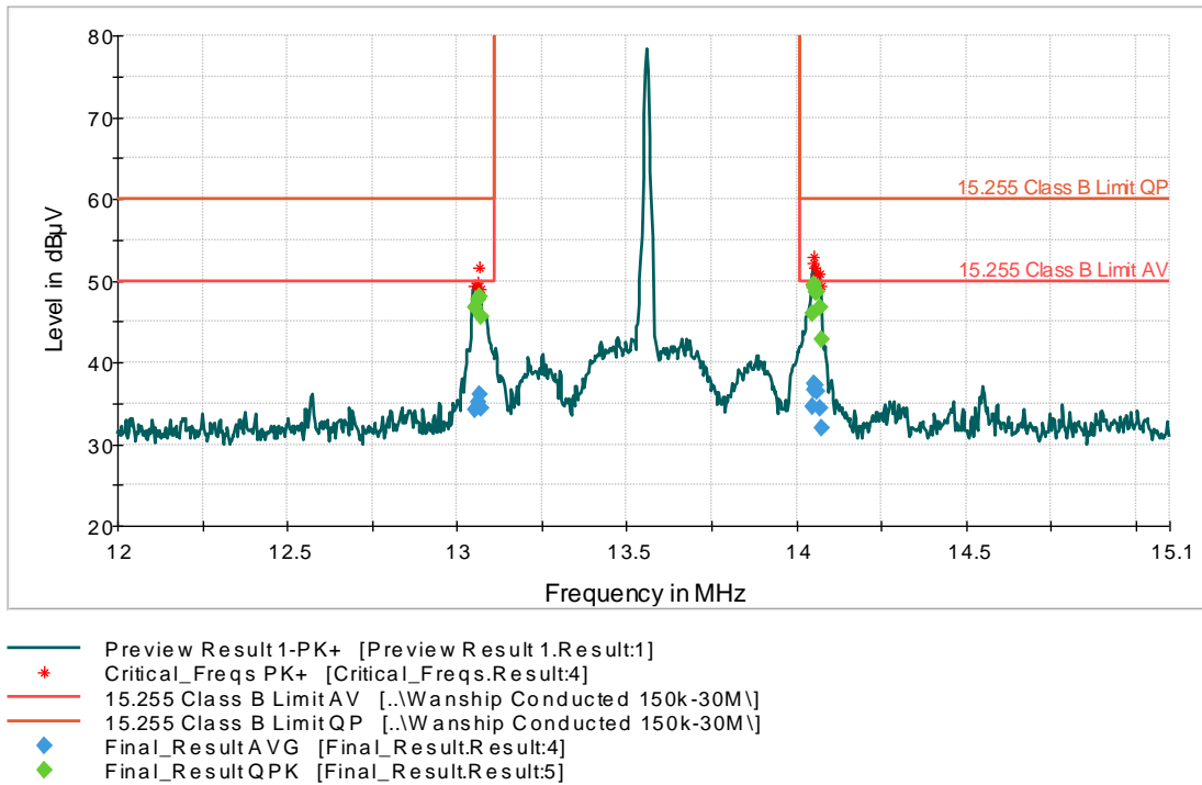
Graph 4: AC Mains Conducted Hot Lead Fundamental Emission Band Edges without Tags – Antenna 2 Transmitting
