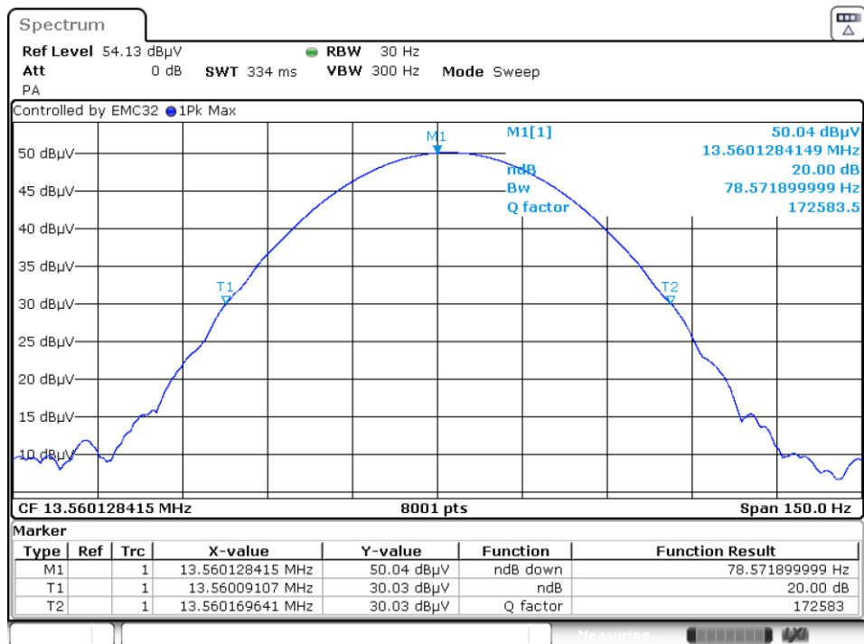
Graph 9: Worst-Case 20dB Bandwidth (Antenna 1 Transmitting)
