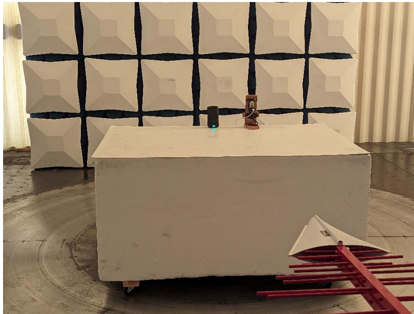
Photograph 3: Front View Radiated Emissions Worst-Case Configuration – Frequencies 30-1000MHz
