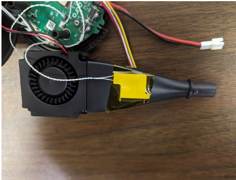
Photograph 25: View of NFC Antenna on Enclosure (One Per Side)
