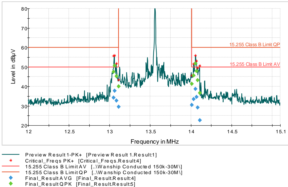
Graph 1: Hot Lead AC Mains Conducted Fundamental Emission Band Edges with Tags - Antenna 1 Transmitting
