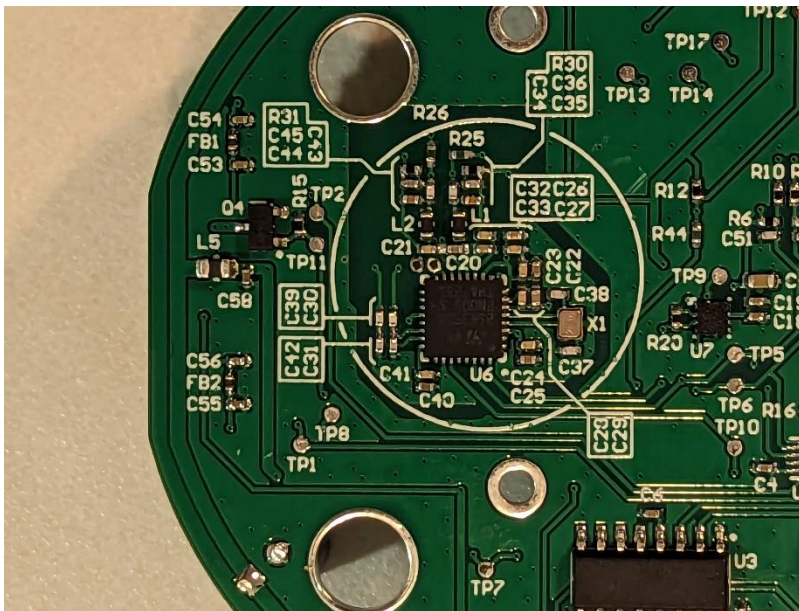
Photograph 24: Close-up View of PCB Section Under Ferrite Plate
