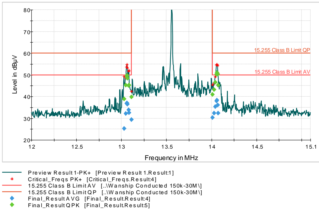
Graph 2: Hot Lead AC Mains Conducted Fundamental Emission Band Edges without Tags - Antenna 1 Transmitting
