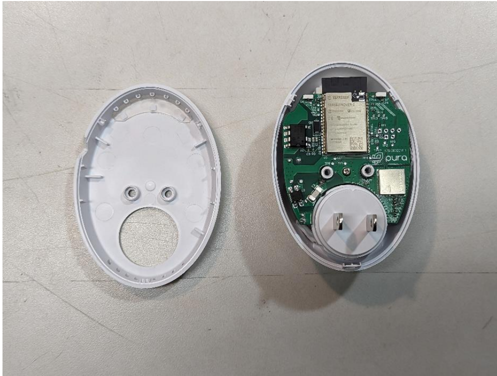
Photograph 5 – View of PCBA in the Housing
