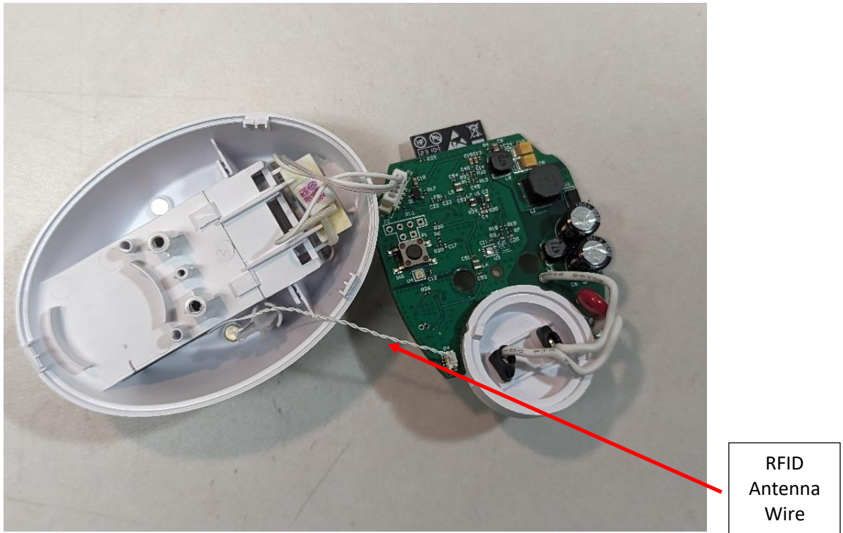
Photograph 6 – View of PCBA in the Housing with Cables and RFID Antenna Connection
