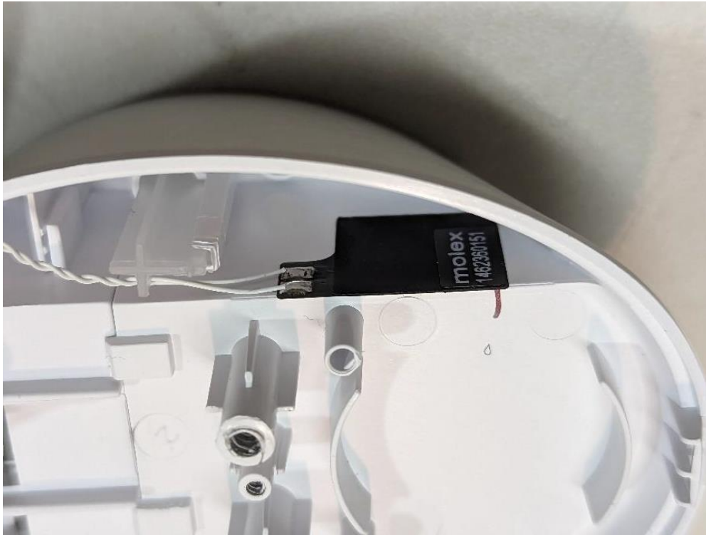
Photograph 7 – View of RFID Antenna Placement in Housing
