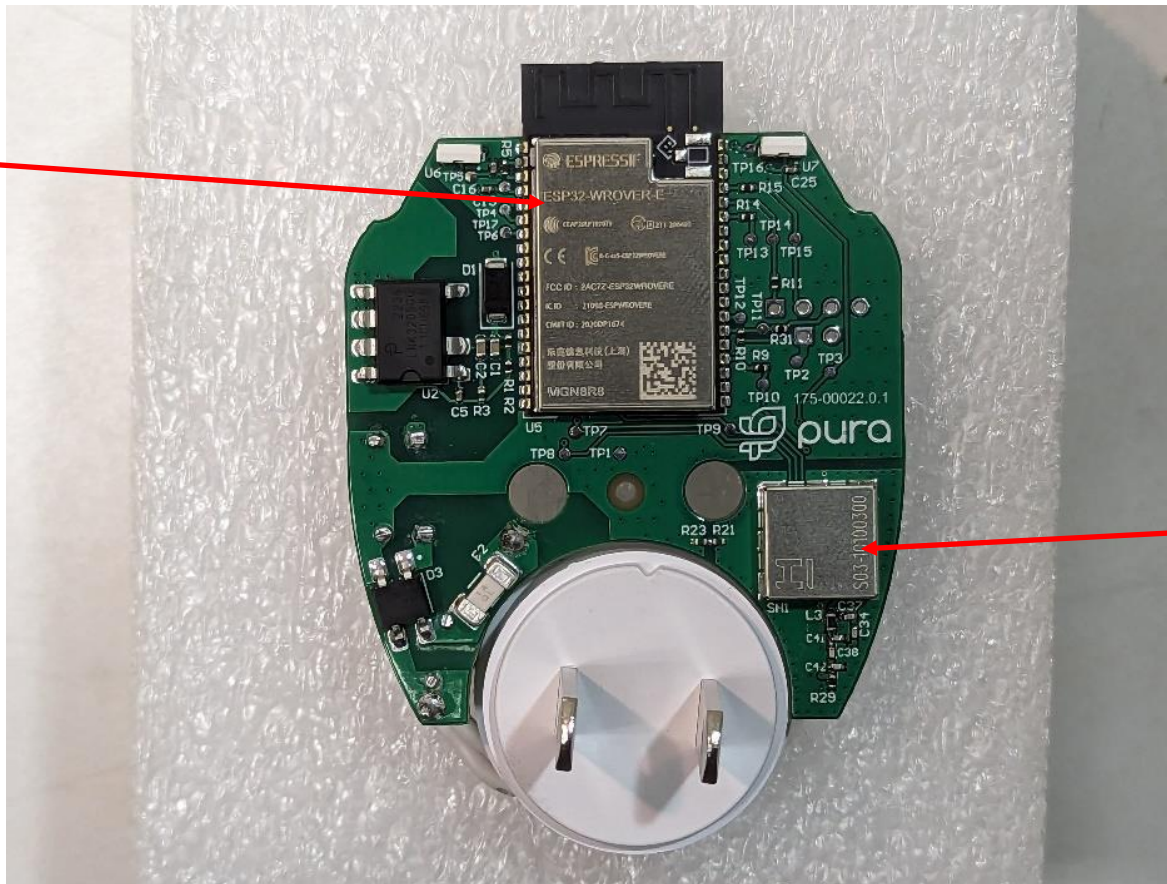
Photograph 1 – Front View of the PCBA
