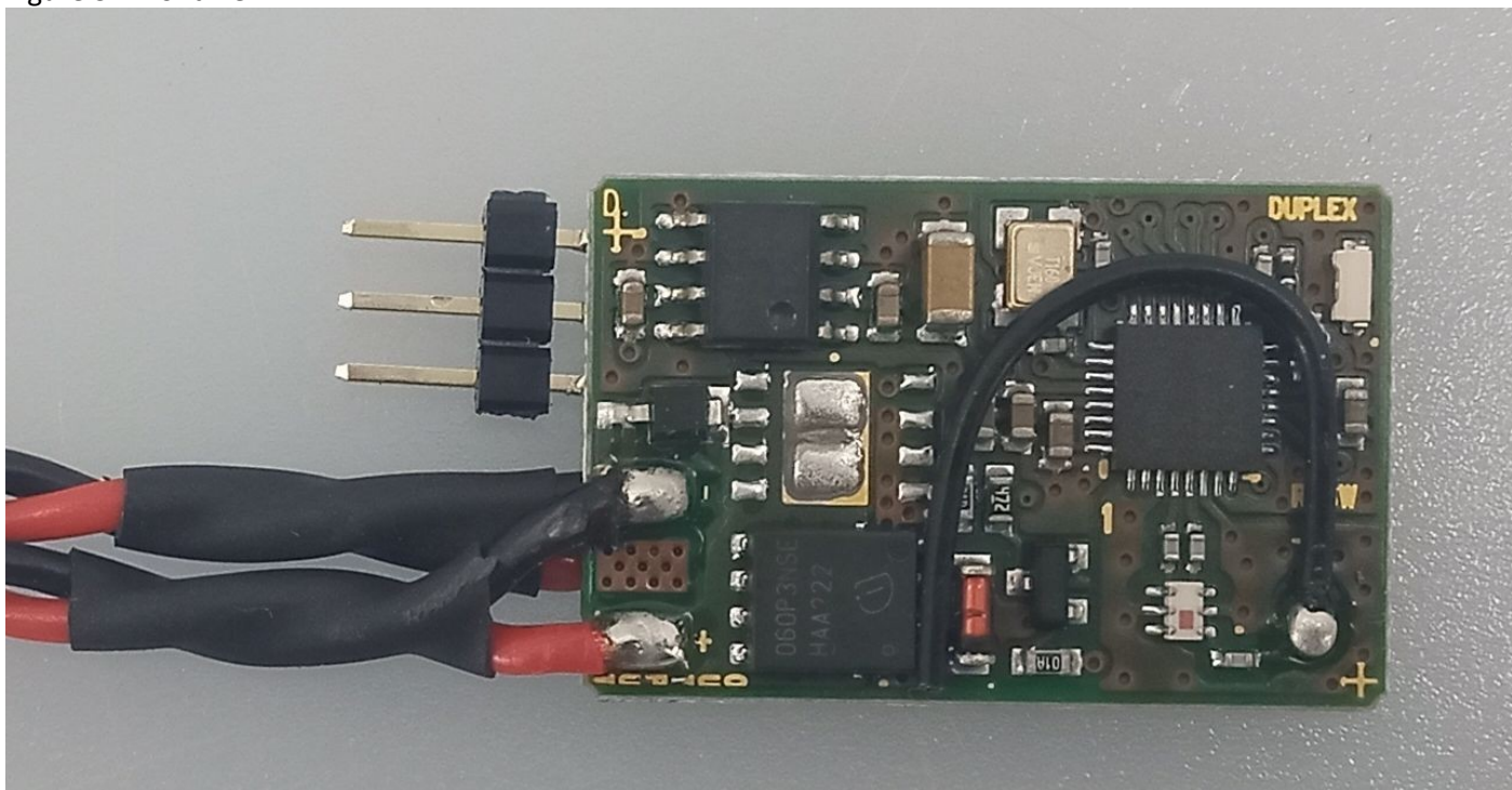
Figure 3 - Front view
