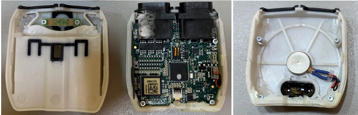
Figure 1 – Enclosure removed
