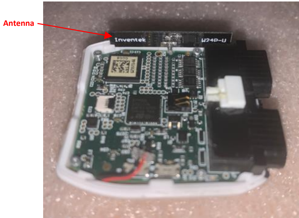
Figure 2 – PCB, Top angled view
