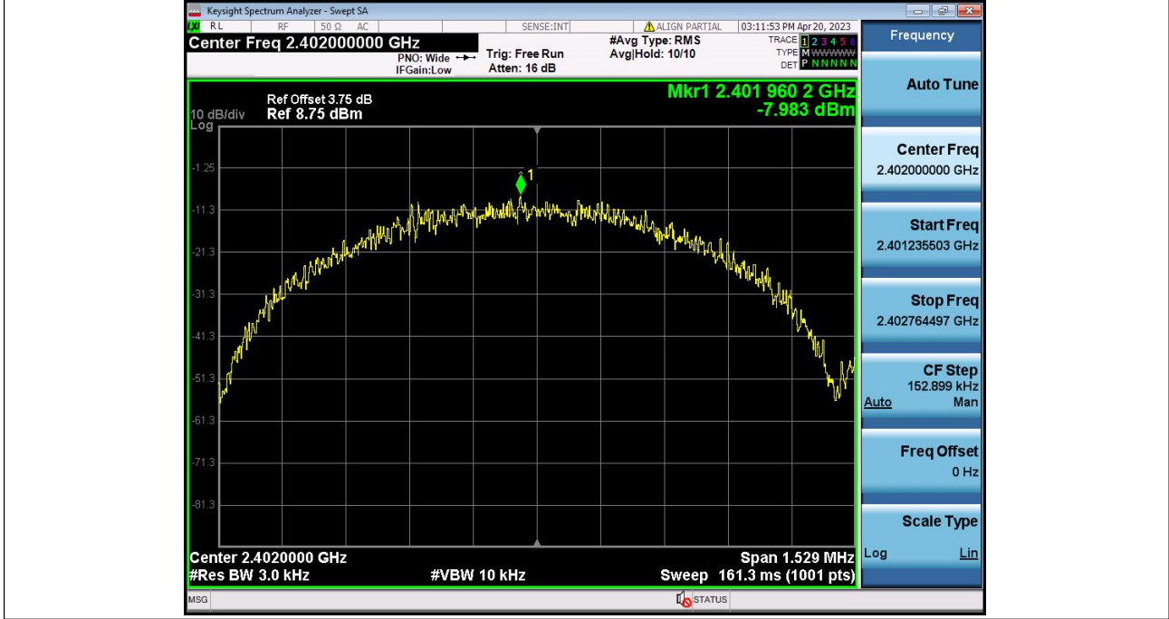
Power Spectral Density_NVNT_ANT1_1Mbps_2402
