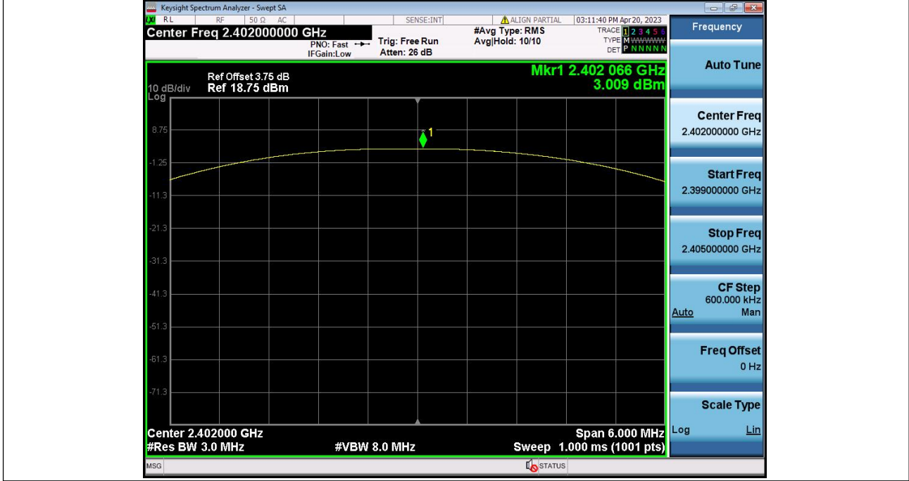
Peak_Output_Power_NVNT_ANT1_1Mbps_2402
