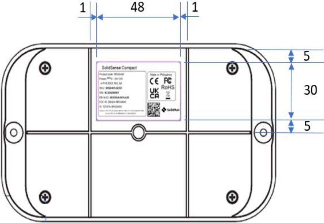
Bottom side of SRG0400
