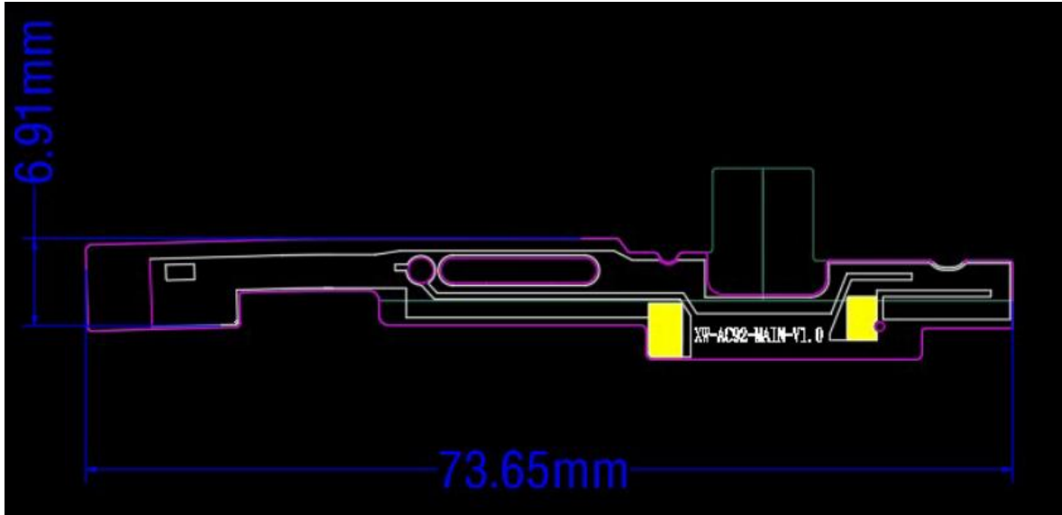
Main antenna
