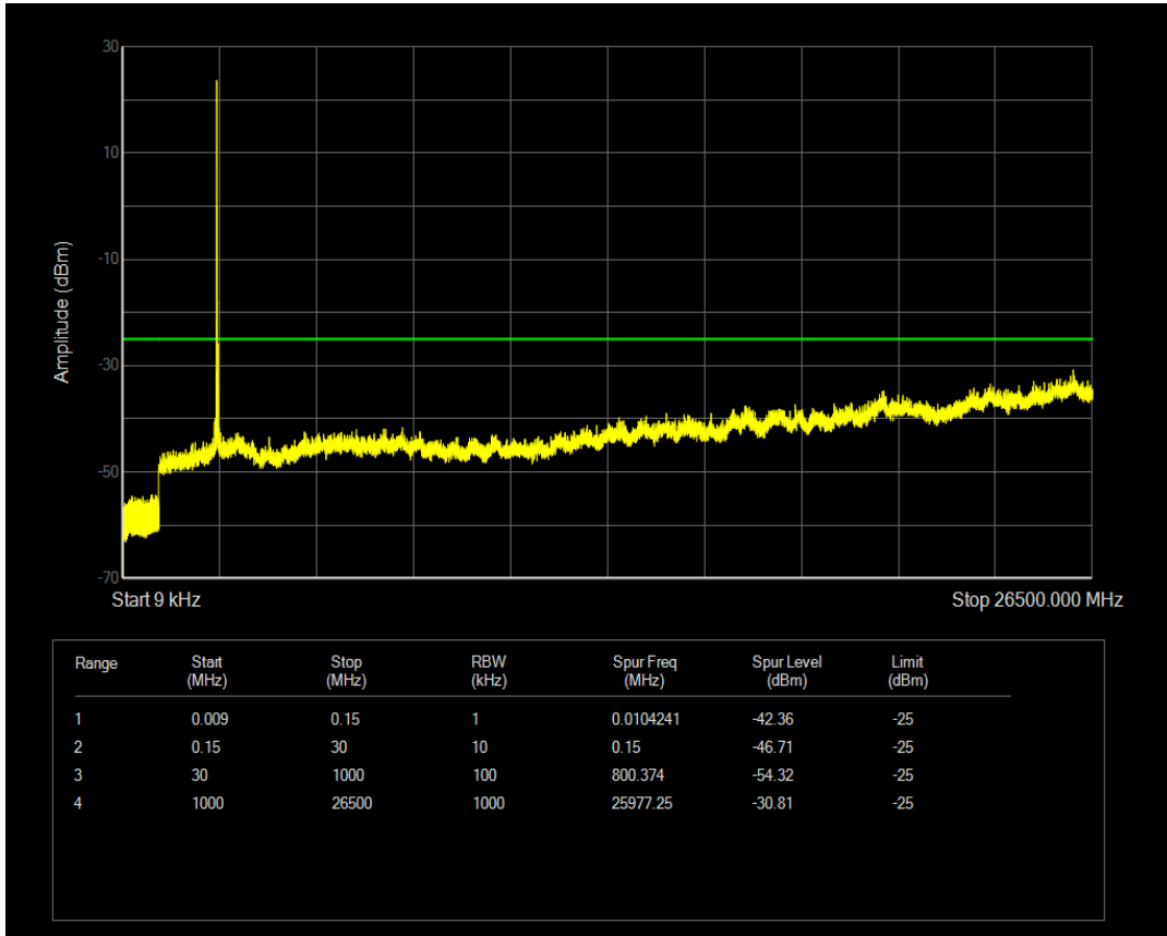
Band41a QPSK BW=20MHz Channel=40640 RB Size=100 Position=#0
