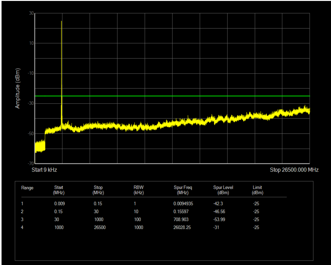
Band41a 16QAM BW=20MHz Channel=40640 RB Size=100 Position=#0
