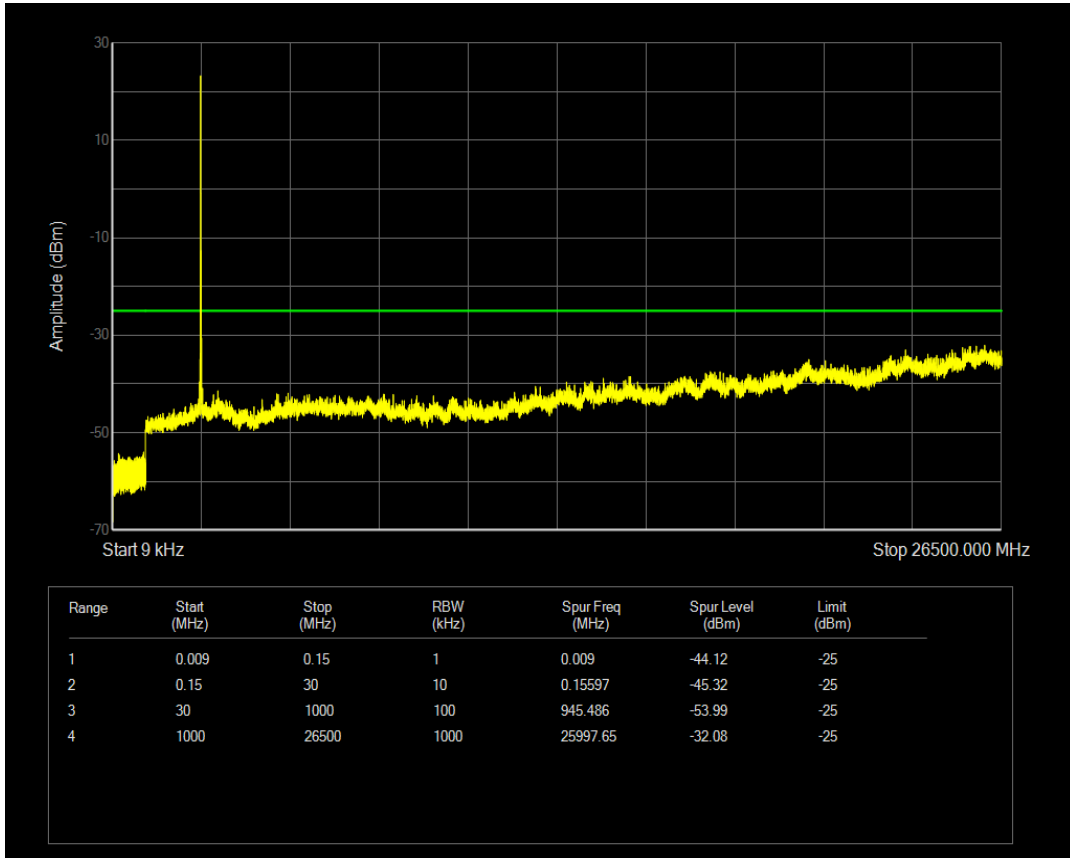
Band41a 16QAM BW=15MHz Channel=41165 RB Size=75 Position=#0
