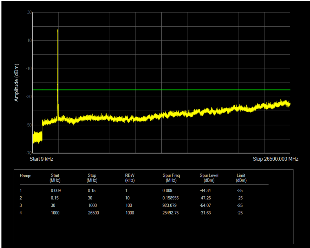
Band41a 16QAM BW=15MHz Channel=40640 RB Size=75 Position=#0
