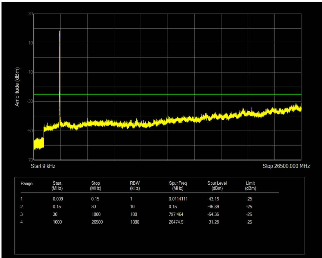
Band41a 16QAM BW=20MHz Channel=40140 RB Size=1 Position=#0
