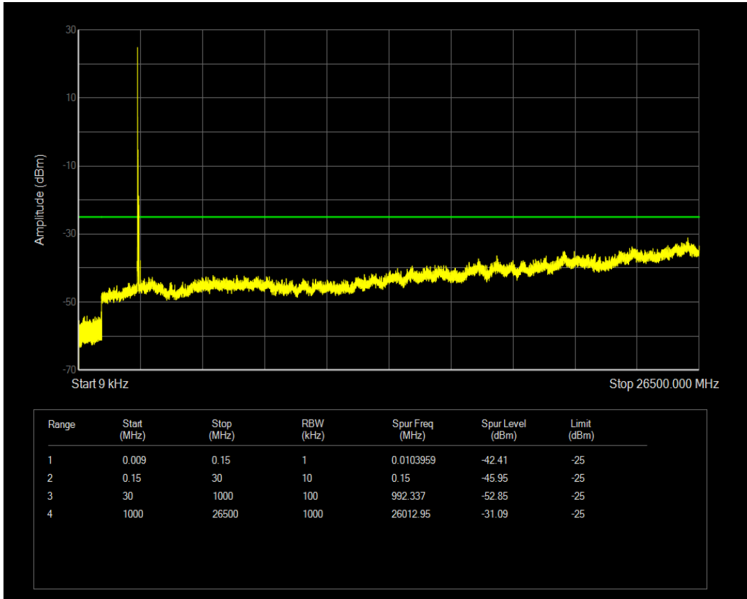
Band41a QPSK BW=20MHz Channel=40140 RB Size=100 Position=#0
