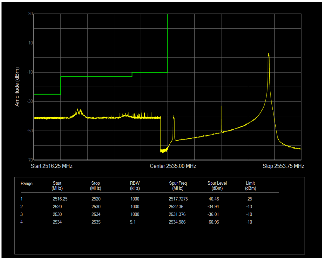
Band41a 16QAM BW=15MHz Channel=40115 RB Size=75 Position=#0
