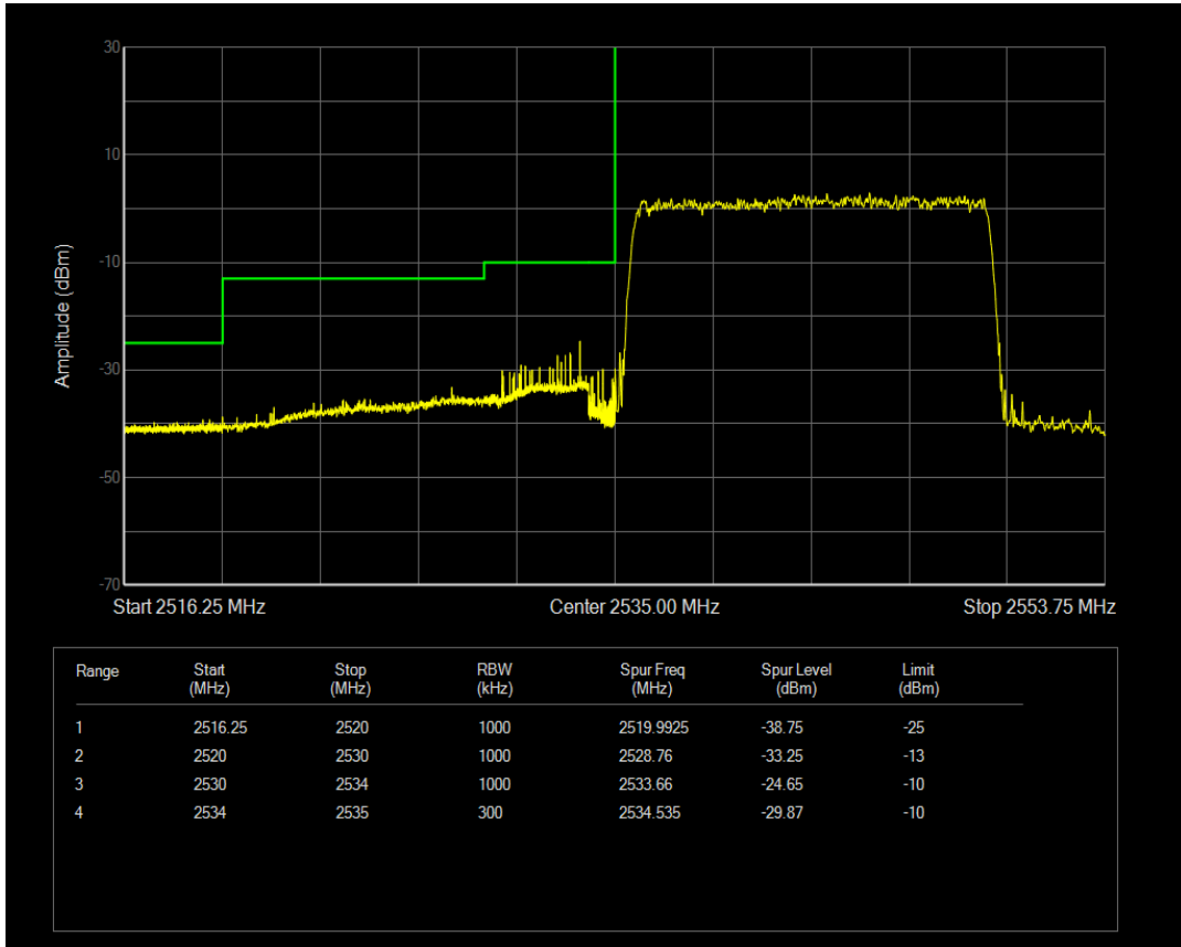
Band41a QPSK BW=15MHz Channel=40115 RB Size=1 Position=#Max
