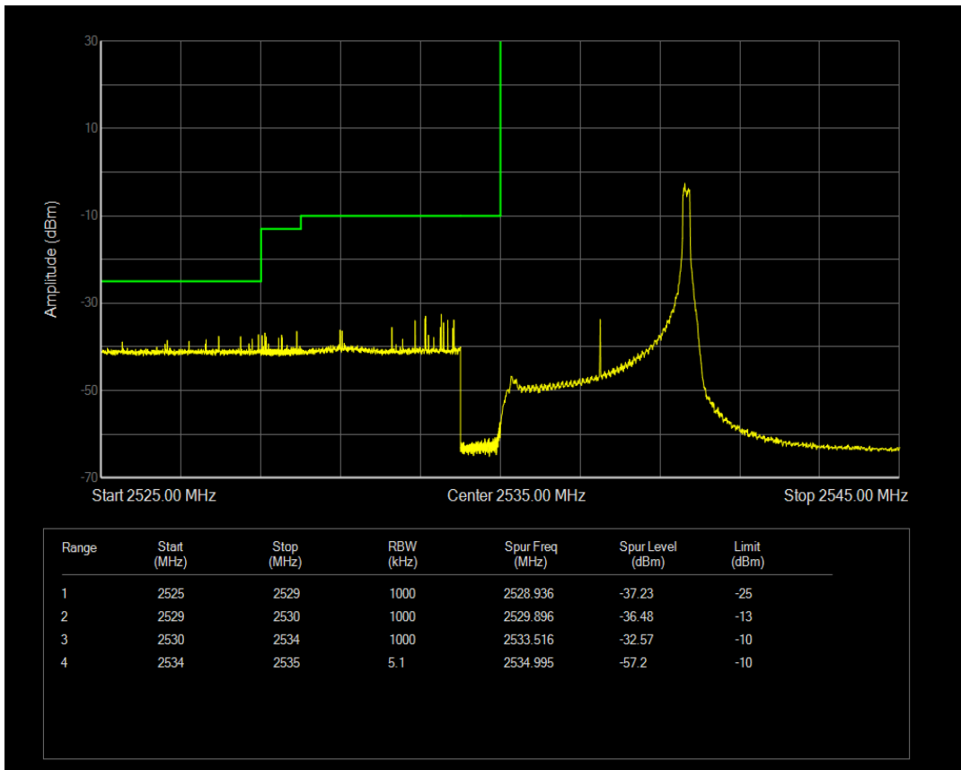
Band41a 16QAM BW=5MHz Channel=40065 RB Size=25 Position=#0
