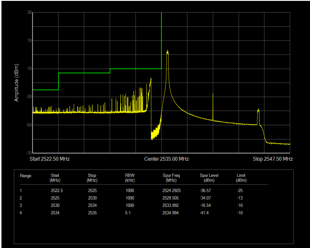
Band41a 16QAM BW=10MHz Channel=40090 RB Size=1 Position=#Max
