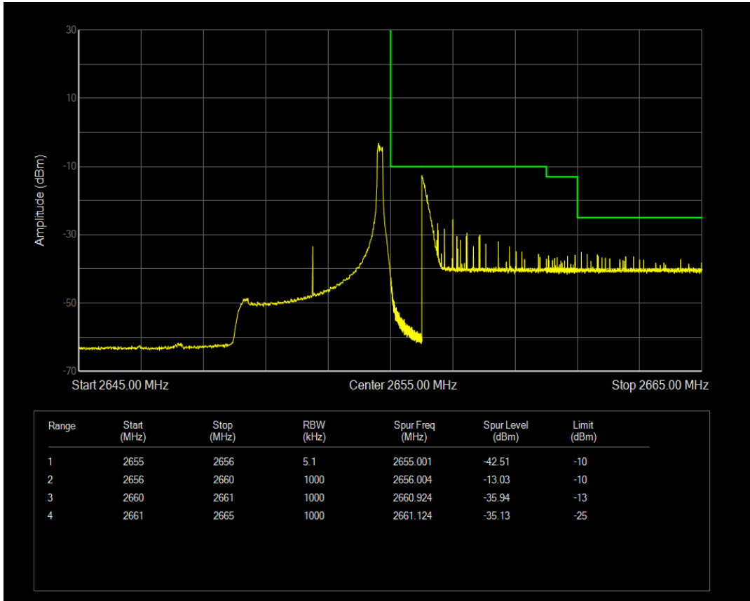
Band41a 16QAM BW=5MHz Channel=41215 RB Size=1 Position=#0
