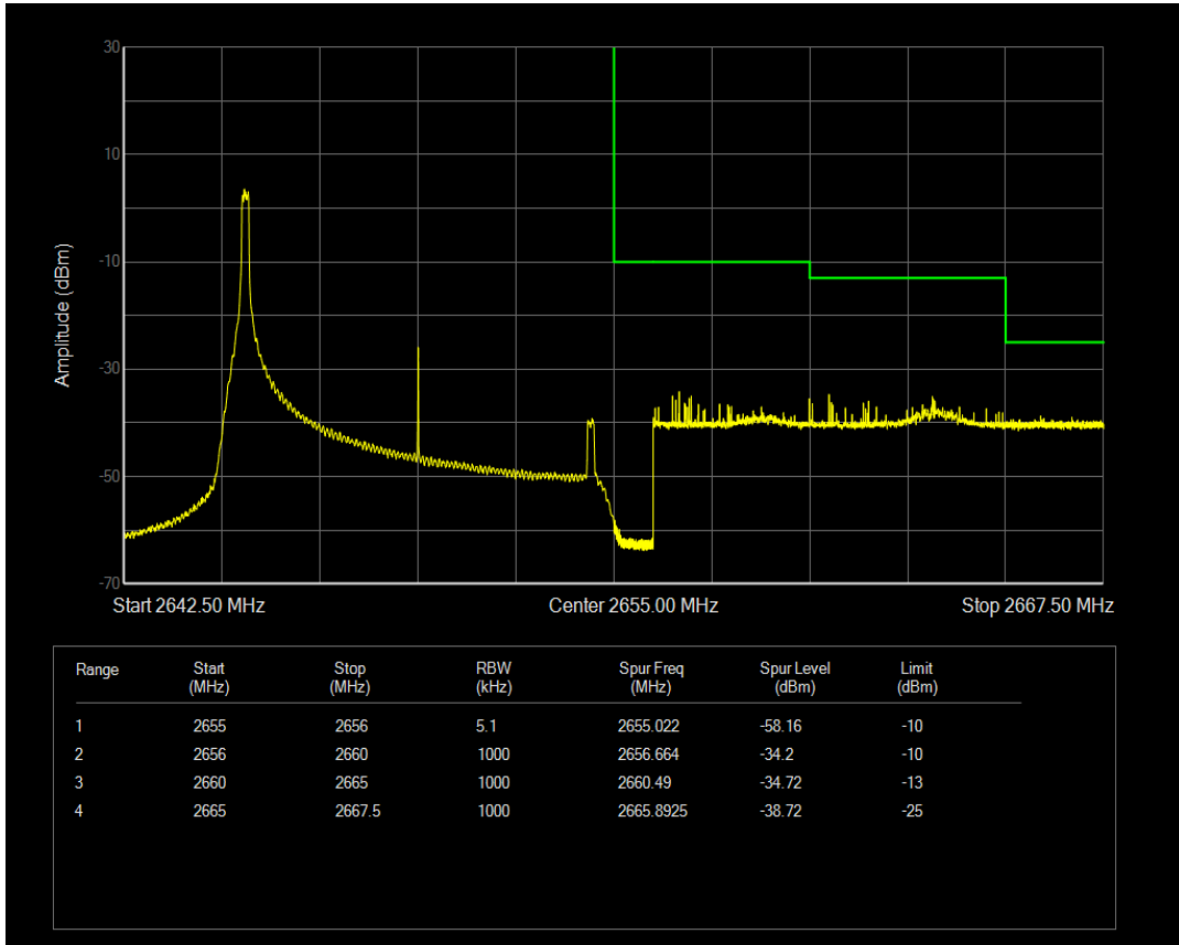
Band41a 16QAM BW=10MHz Channel=41190 RB Size=1 Position=#Max
