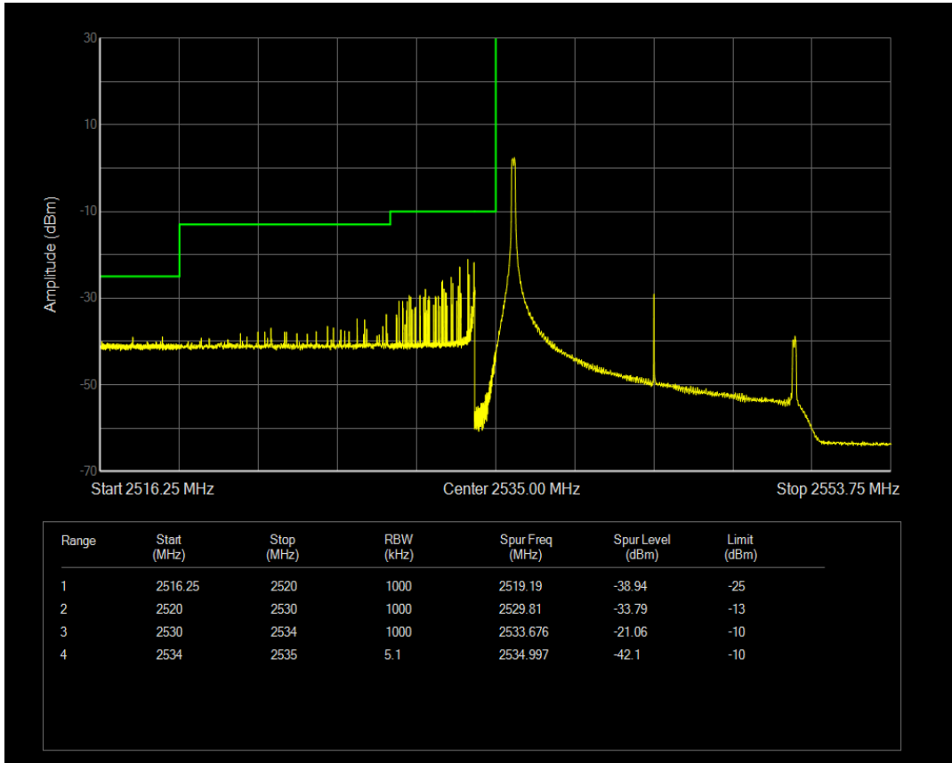
Band41a 16QAM BW=15MHz Channel=40115 RB Size=1 Position=#Max
