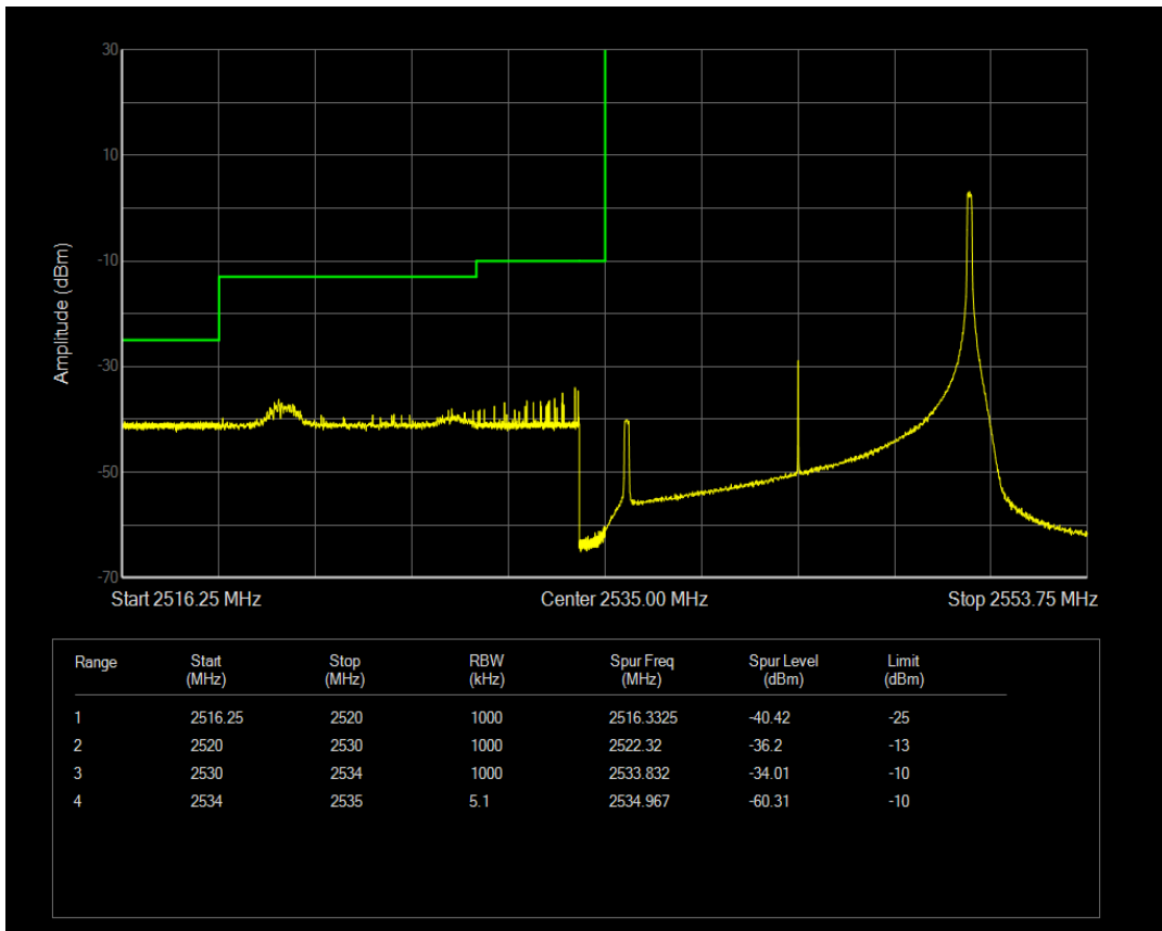
Band41a 16QAM BW=15MHz Channel=40115 RB Size=1 Position=#0
