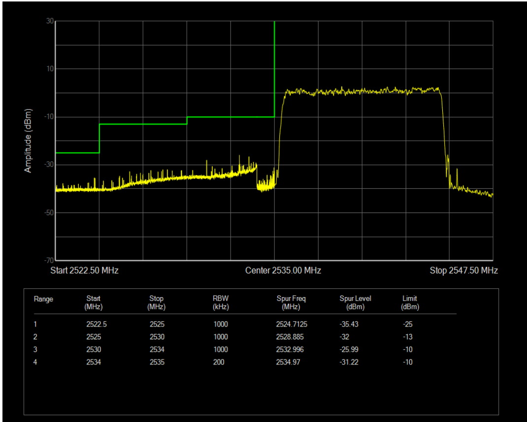
Band41a QPSK BW=10MHz Channel=40090 RB Size=1 Position=#Max
