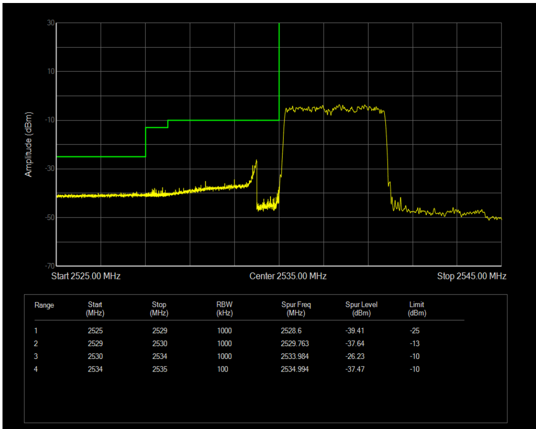
Band41a 16QAM BW=5MHz Channel=40065 RB Size=1 Position=#0
