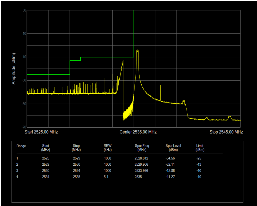
Band41a 16QAM BW=5MHz Channel=40065 RB Size=1 Position=#Max
