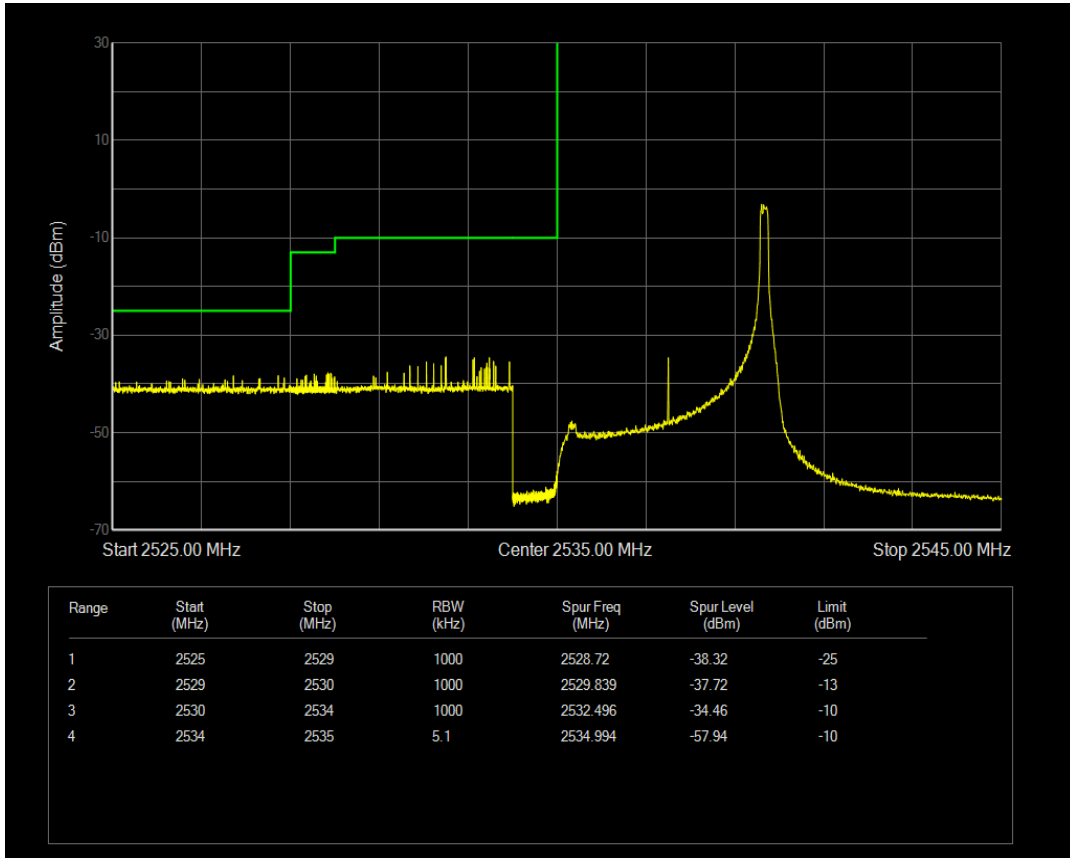
Band41a QPSK BW=5MHz Channel=40065 RB Size=25 Position=#0
