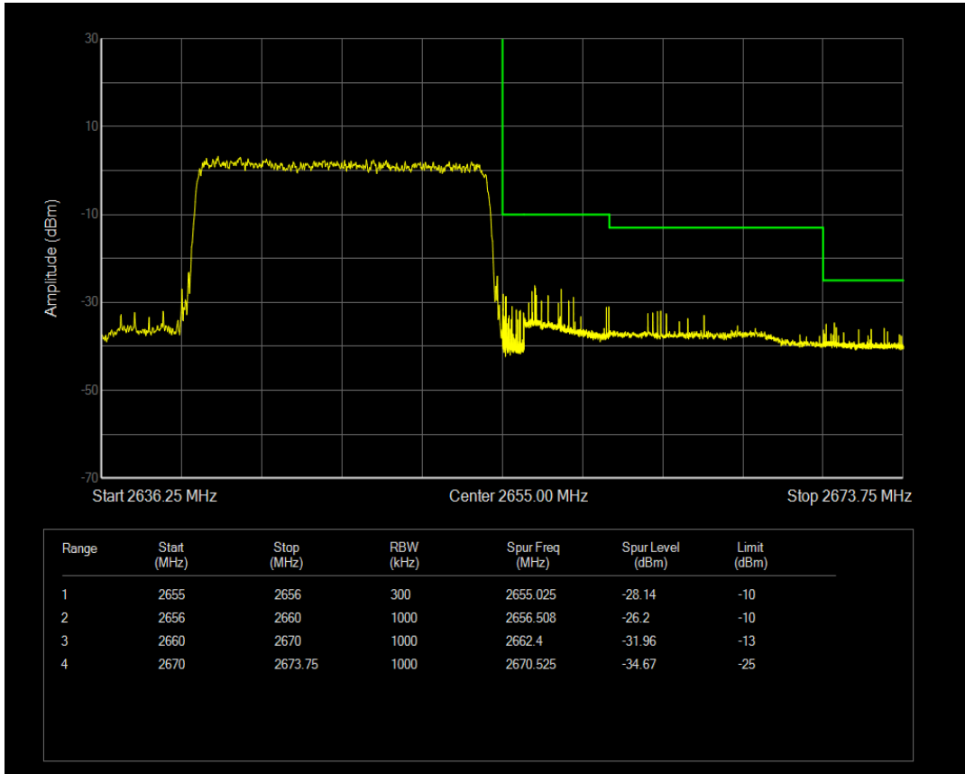
Band41a QPSK BW=15MHz Channel=41165 RB Size=1 Position=#Max
