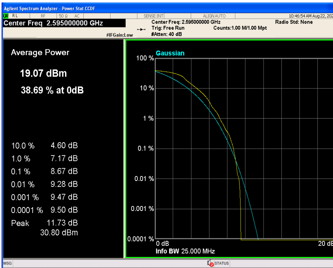
Band41a 16QAM BW=10MHz Channel=40640 RB Size=1 Position=#0
