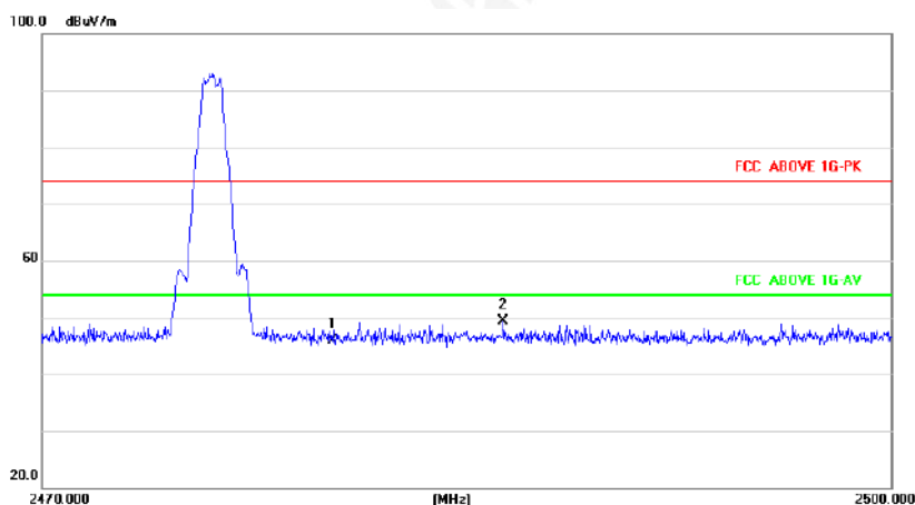
2475MHz Horizontal
