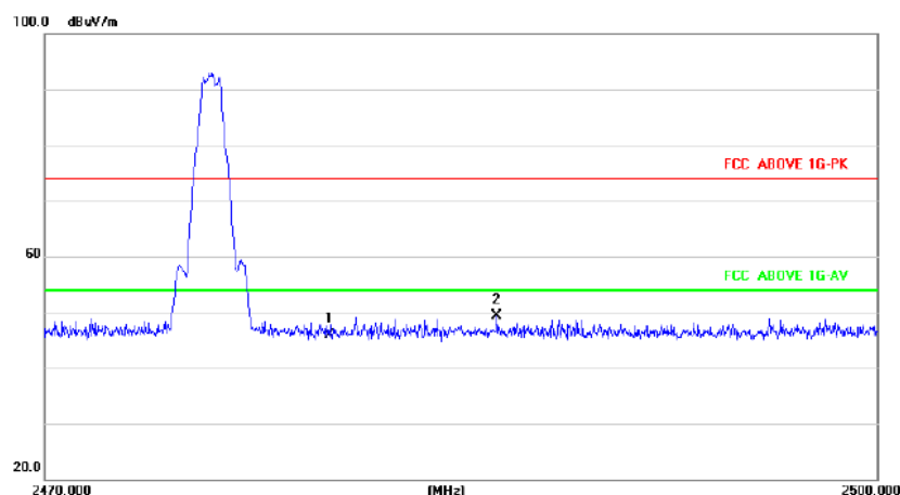
2475MHz Vertical
