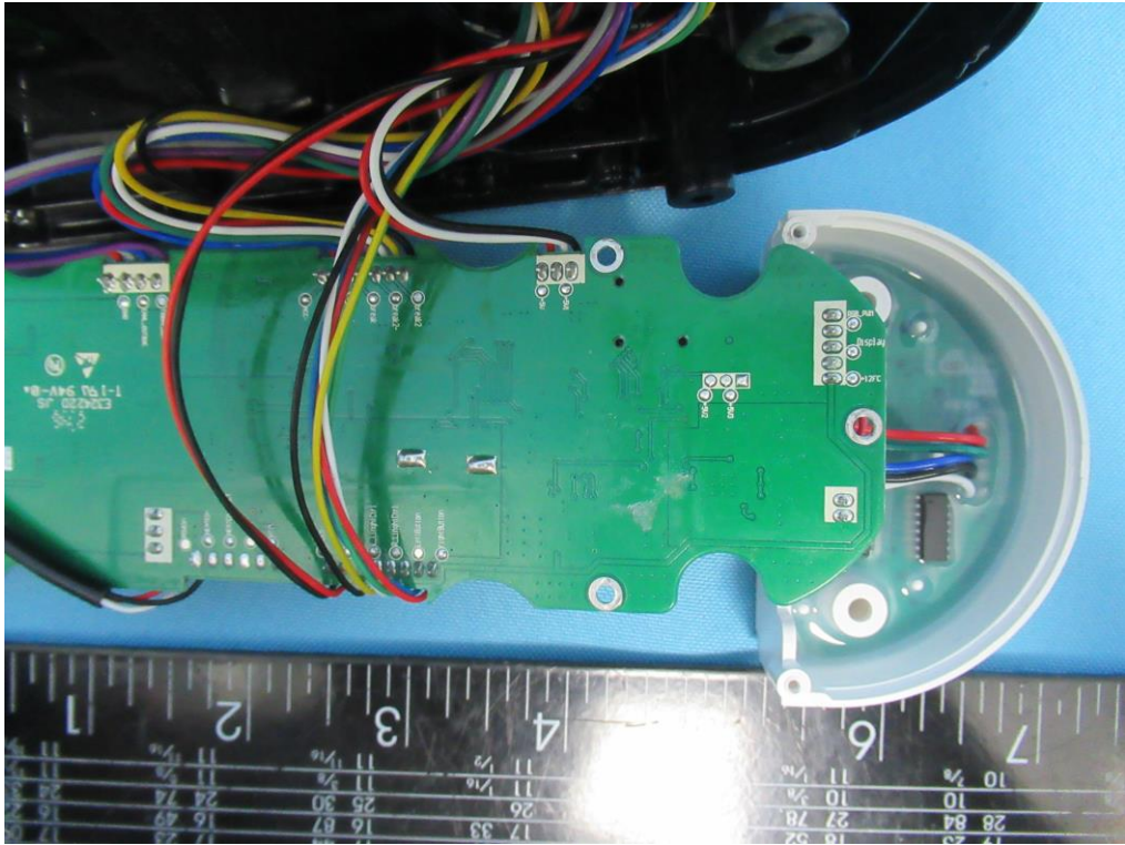
(7) EUT Photo
