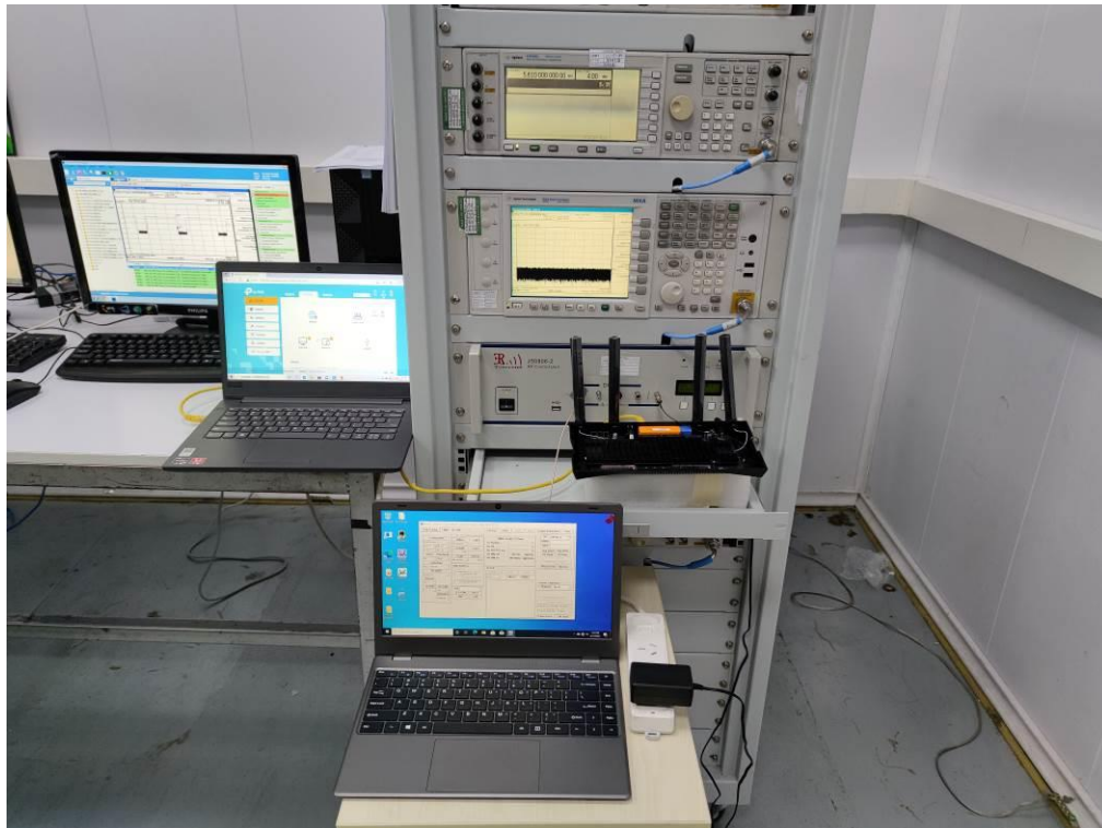
Test Setup Photo of Dynamic Frequency Selection Test
