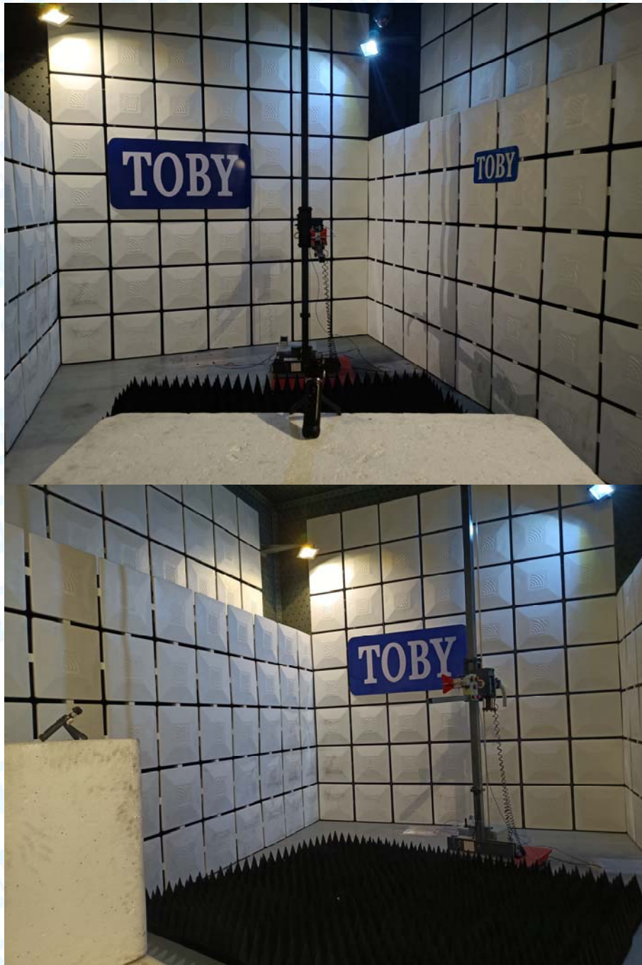
Photo of Setup for Radiated Emission (Above 1 GHz)
