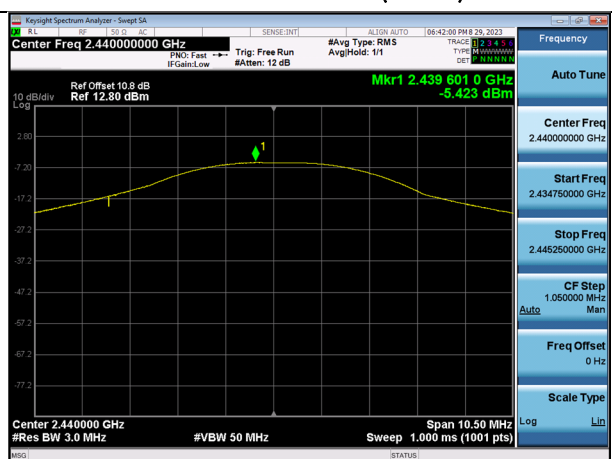
GFSK : Peak Power (CH.20)
