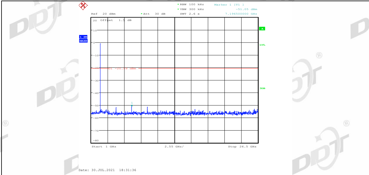
DH5_Ant1_2441_0~Reference
