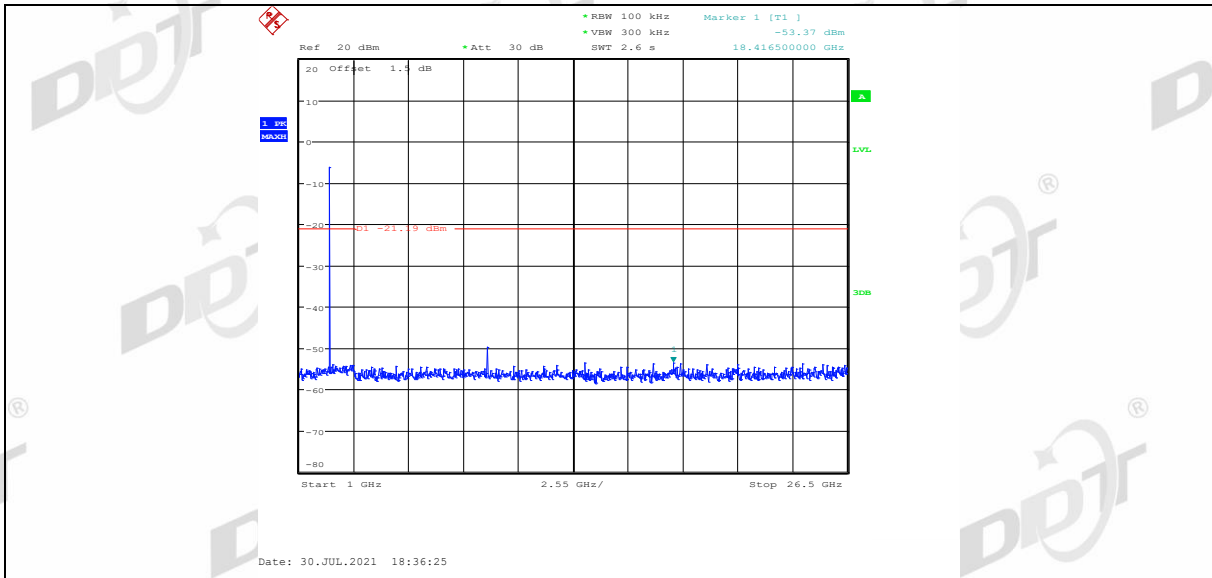
2DH5_Ant1_2480_0~Reference
