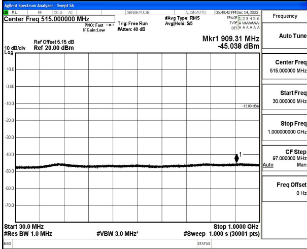
30 MHz – 1000 MHz
