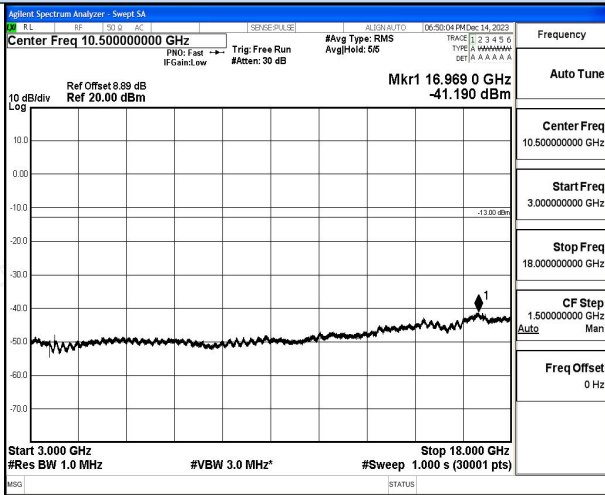
3 GHz – 18 GHz
