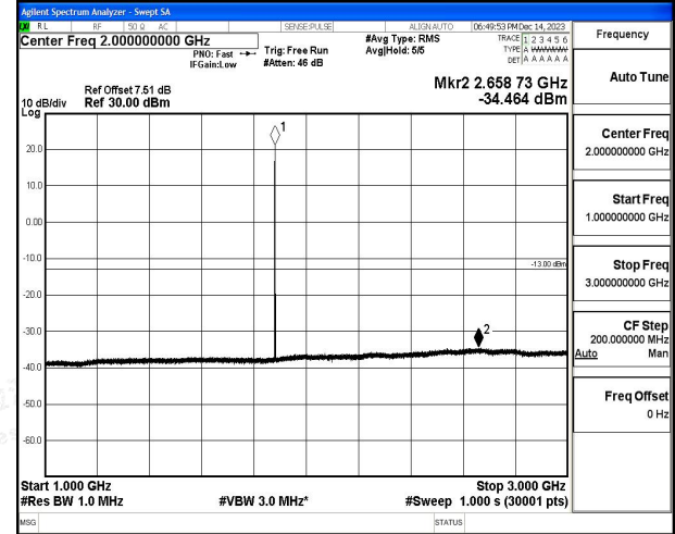
1 GHz – 3 GHz
