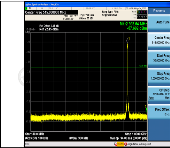
30MHz~1GHz Channel:
