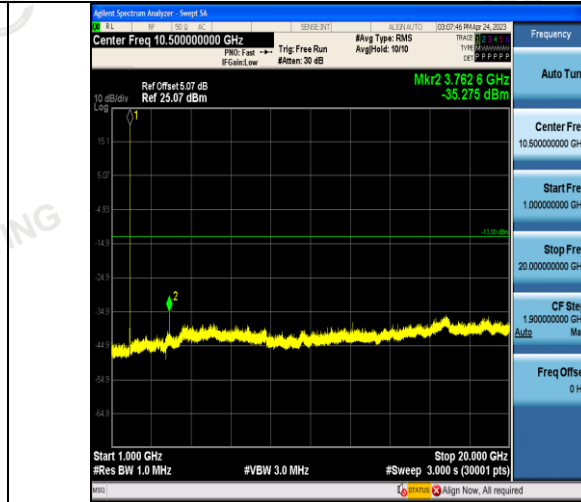
1GHz~20GHz 9538
