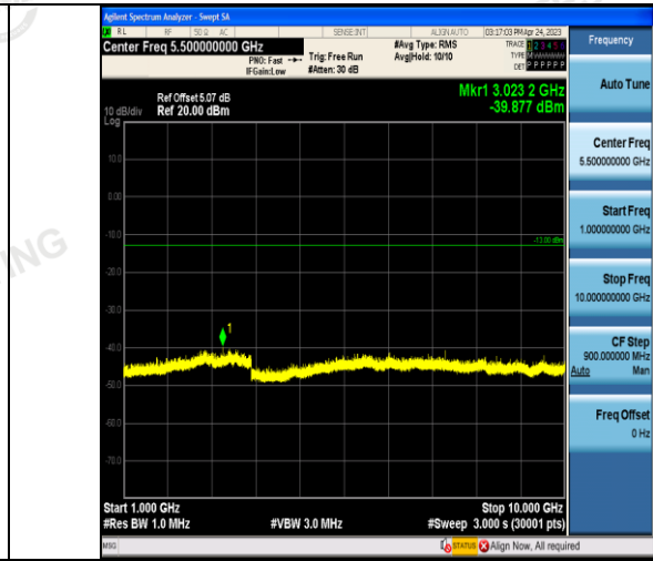
1GHz~10GHz 4233
