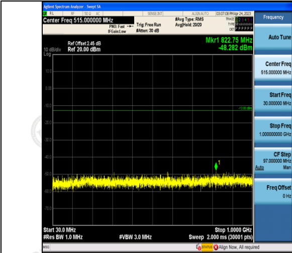
30~1GHz Channel:
