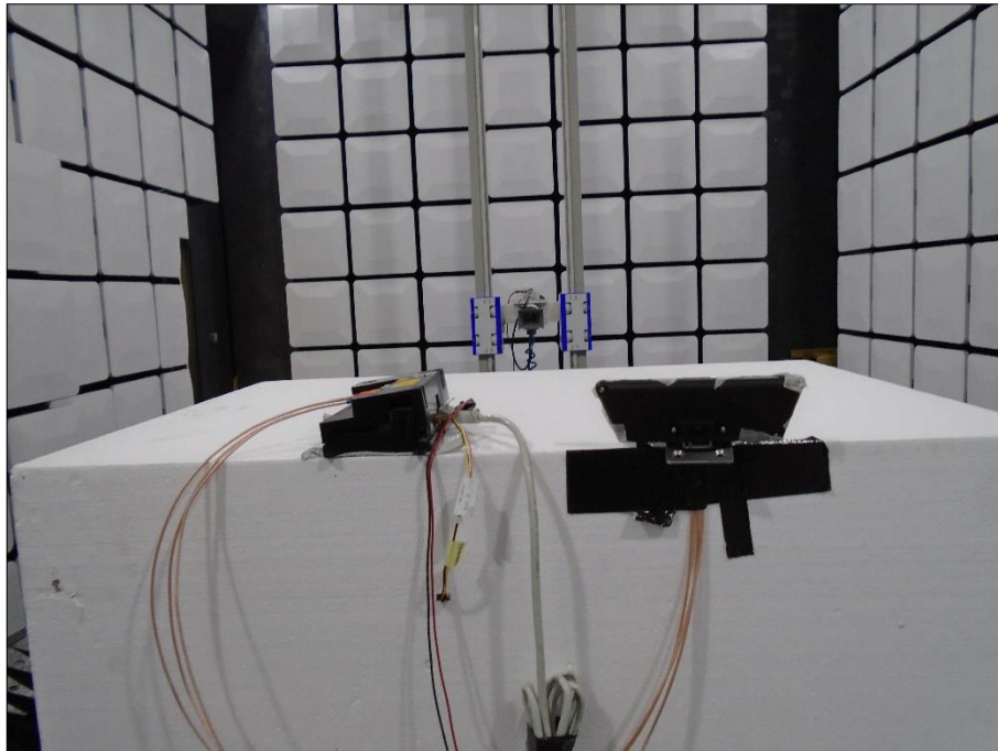
Figure 3 - Test Setup - 8 GHz to 18 GHz
