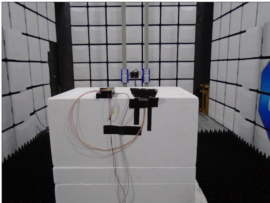
Figure 2 - Test Setup - 1 GHz to 8 GHz
