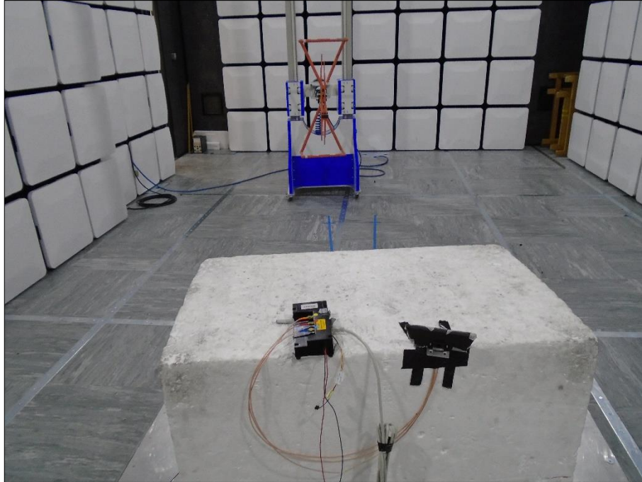
Figure 1 - Test Setup - 30 MHz to 1 GHz
