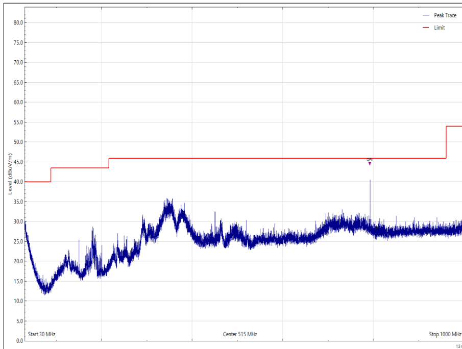
Figure 3 - 2412 MHz, 30 MHz to 1 GHz, Horizontal
