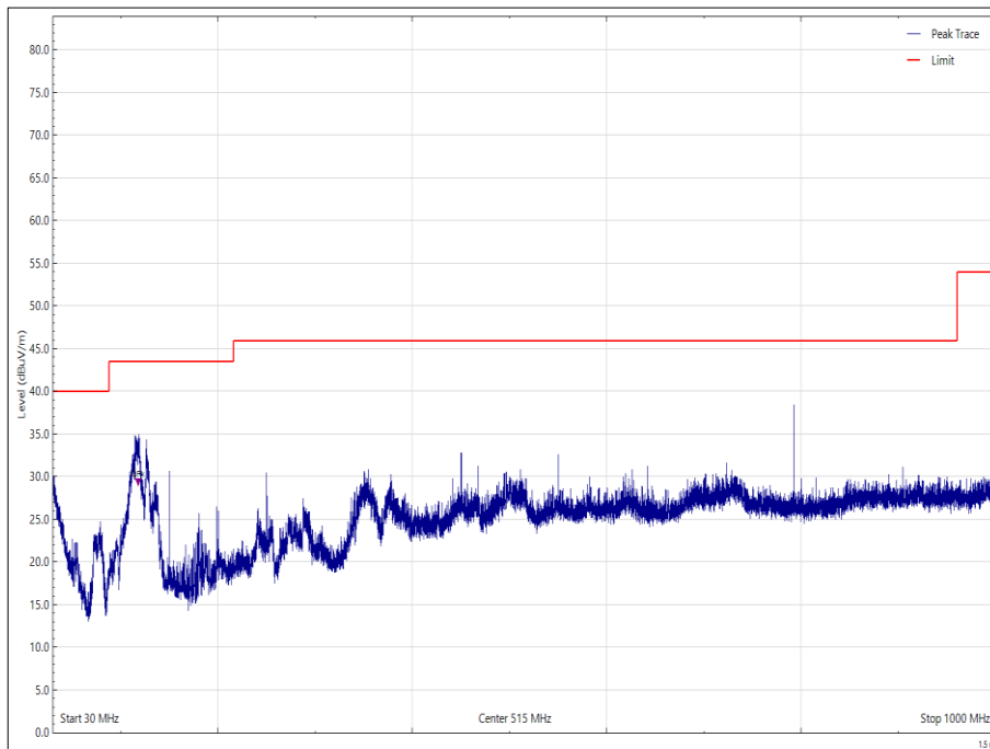
Figure 2 - 2412 MHz, 30 MHz to 1 GHz, Vertical
