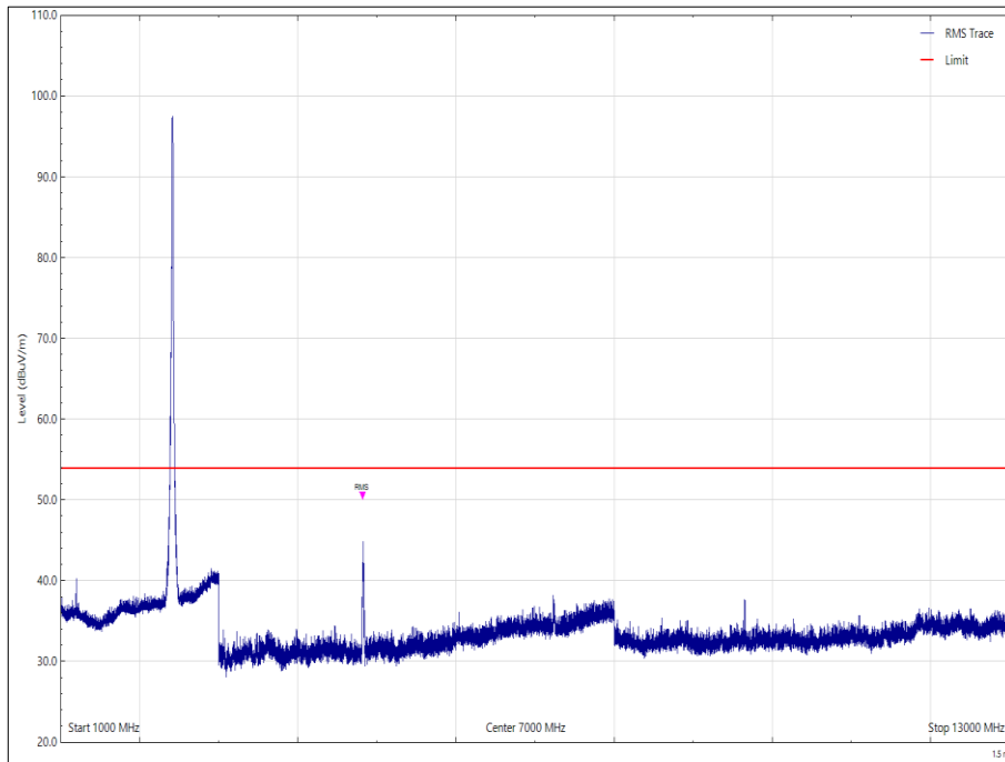
Figure 7 - 2412 MHz, 1 GHz to 13 GHz, Horizontal - Average
