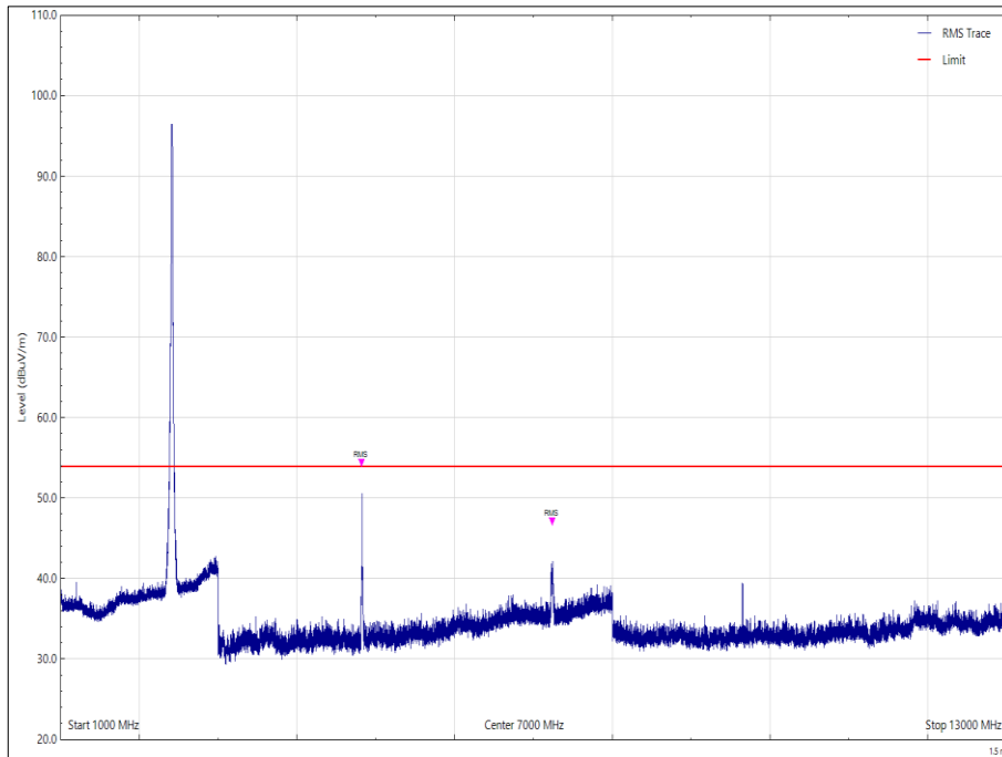
Figure 5 - 2412 MHz, 1 GHz to 13 GHz, Vertical - Average
