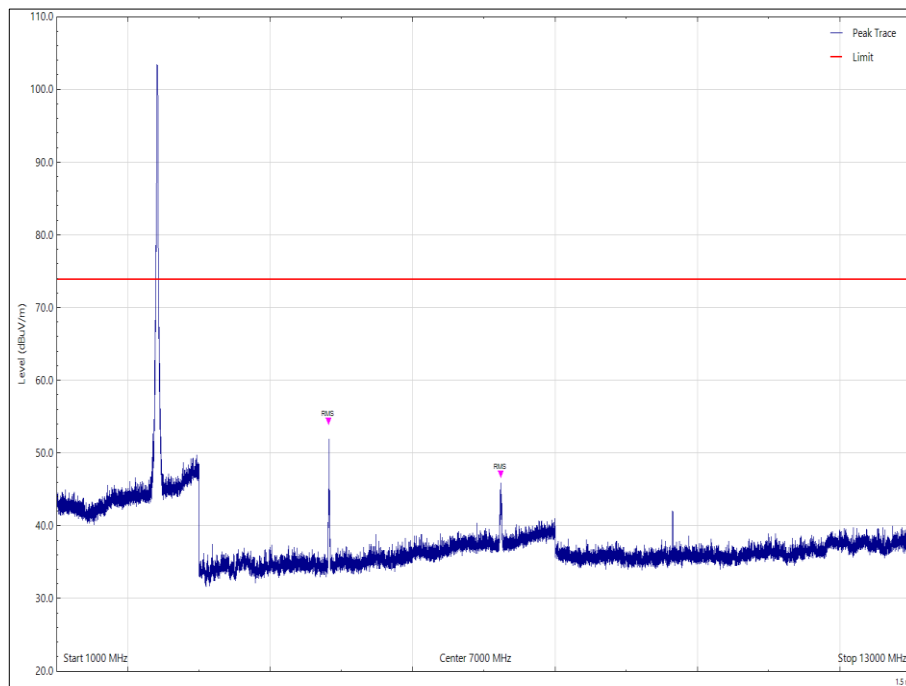
Figure 4 - 2412 MHz, 1 GHz to 13 GHz, Vertical - Peak
