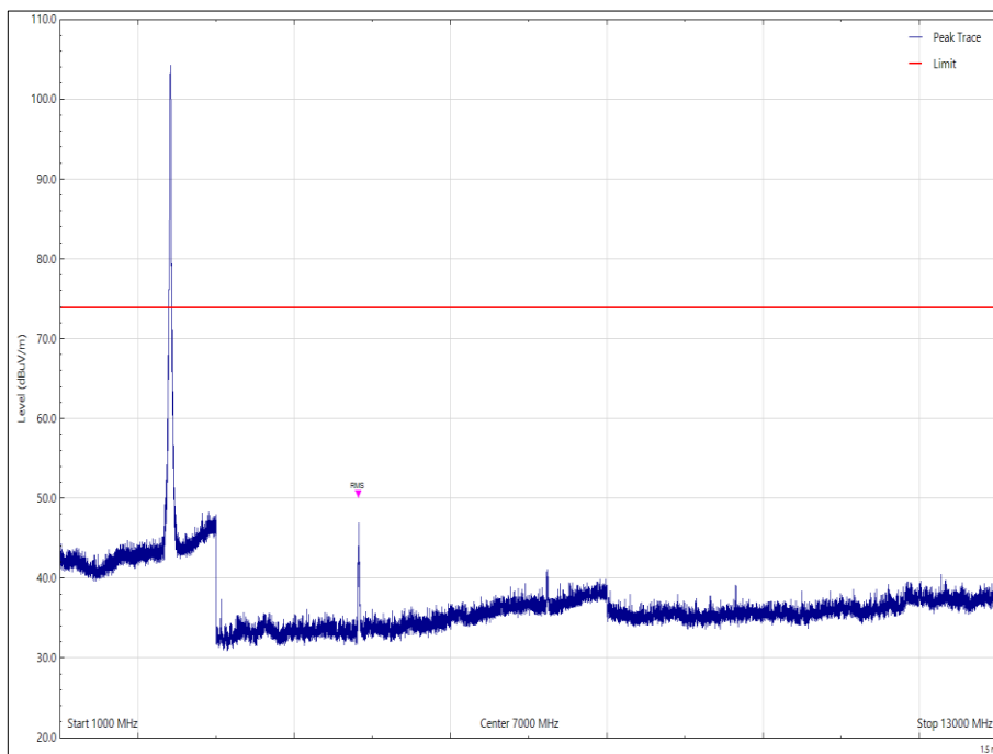
Figure 6 - 2412 MHz, 1 GHz to 13 GHz, Horizontal - Peak
