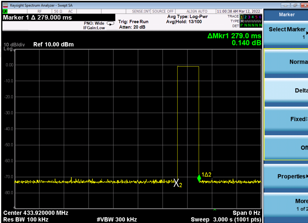
the duration of a transmission Time = 279.0ms=0.279s
