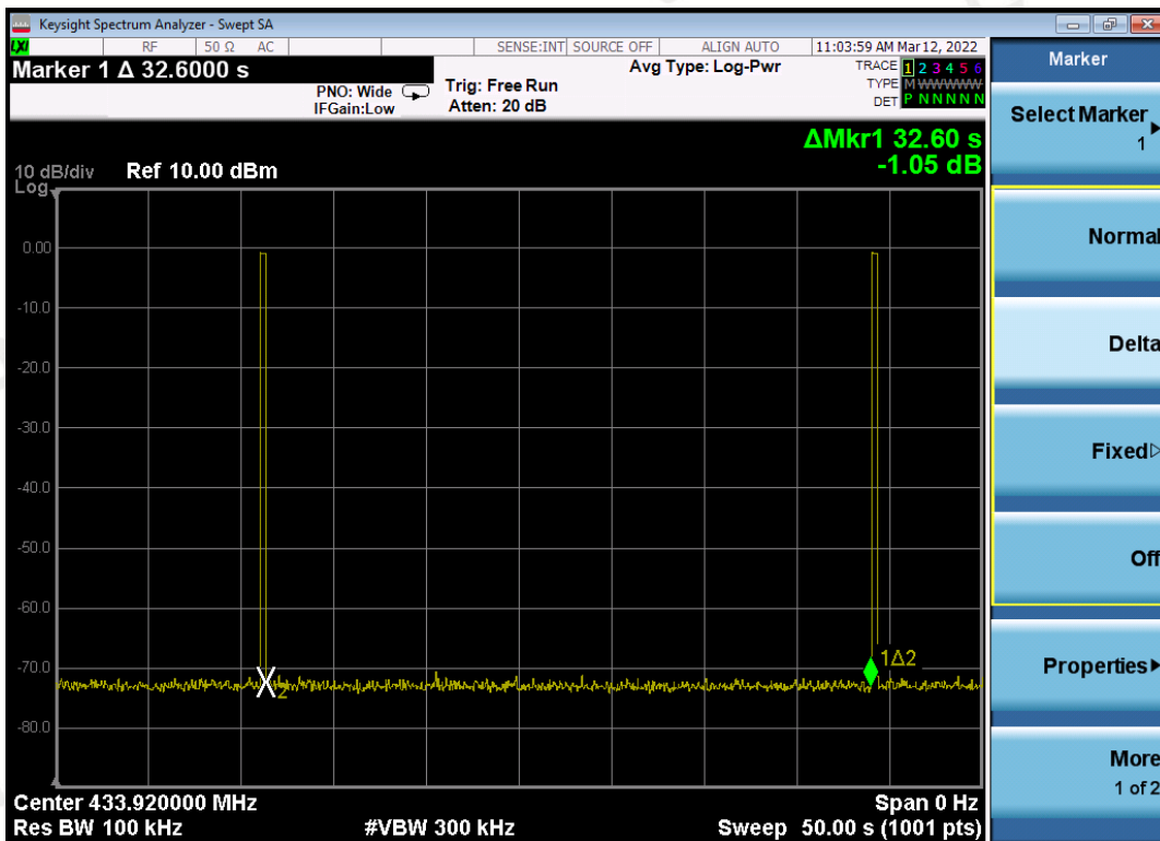
the silent period between transmissions =32.60s
