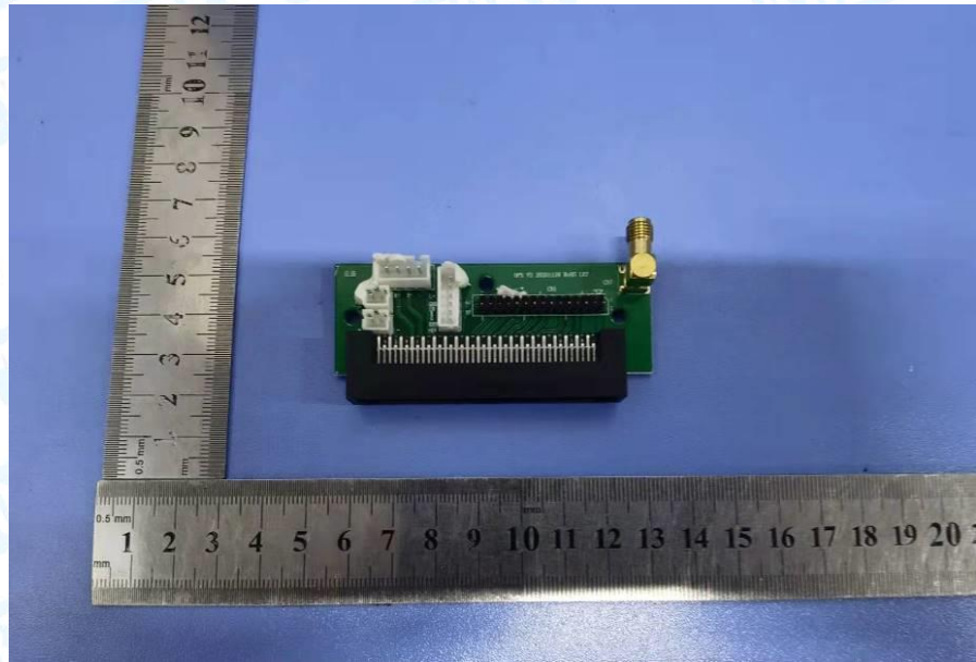
Photo 27 Appearance of PCB
