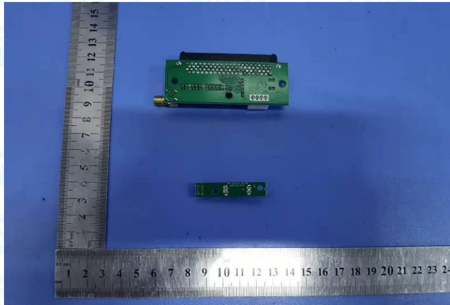
Photo 29 Appearance of PCB
