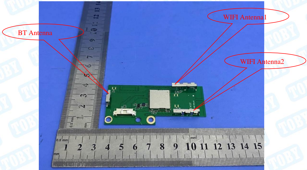
Photo 20 Appearance of PCB
