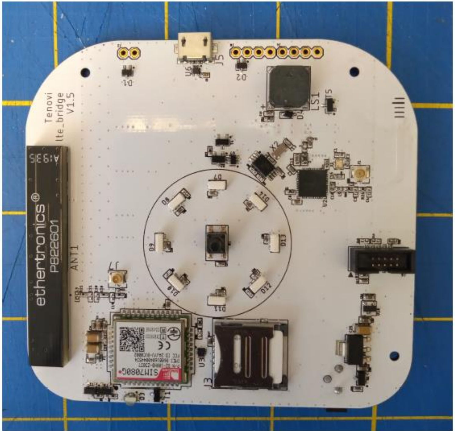
PCB Top View
