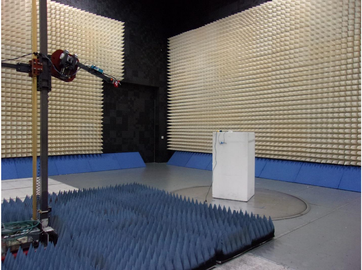
Radiated Emissions 18GHz – 26GHz
