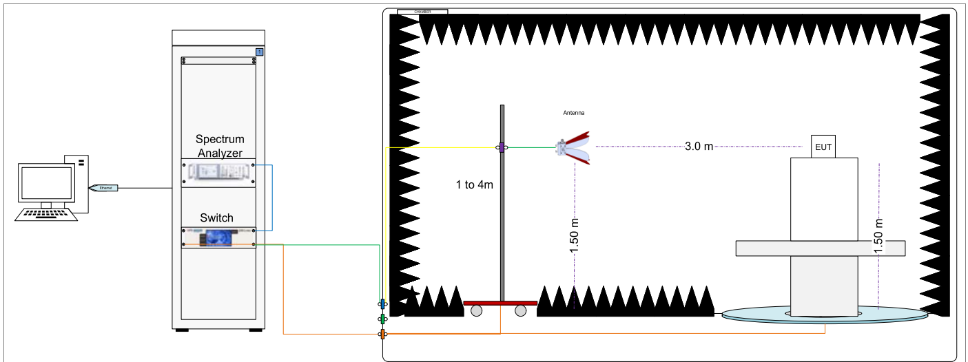
Radiated Setup 9.5 GHz - 18 GHz (Transmitter tests)
