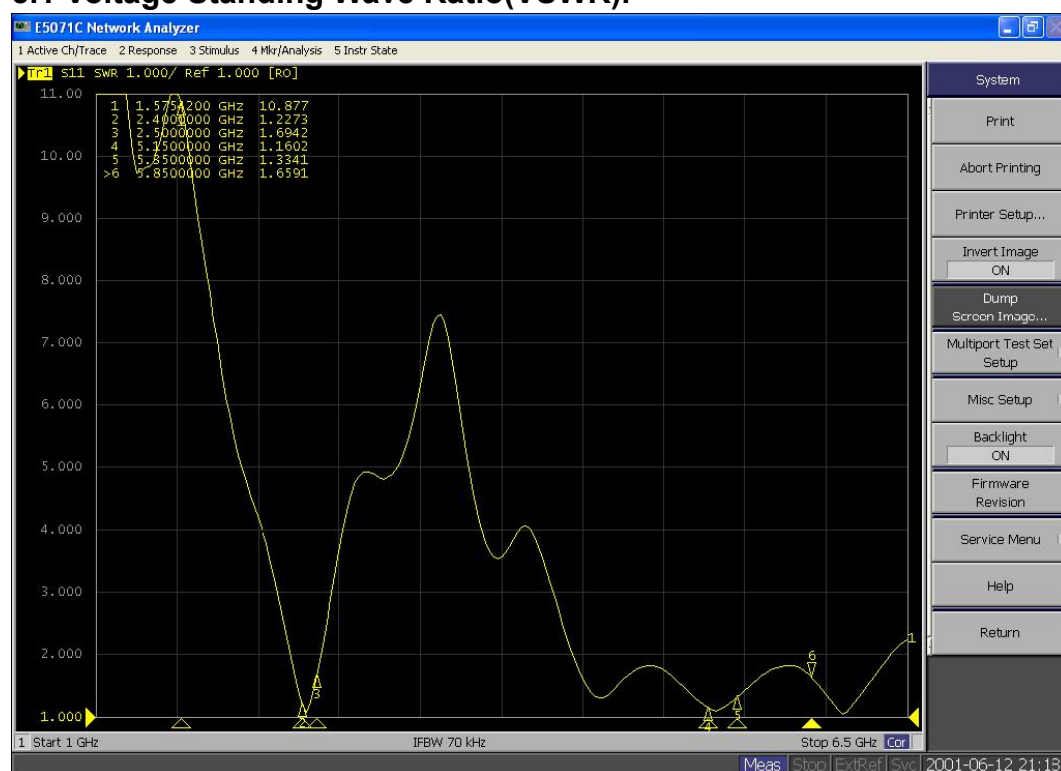
Chart 2 VSWR
