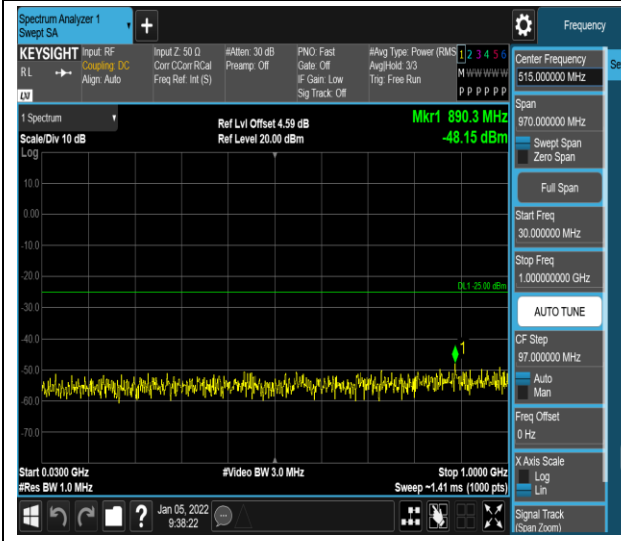
Band7-20MHz-16QAM-21100-1RB#0-Range1:30~1000MHz
