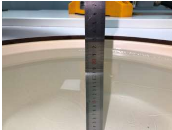
Fig. 9.2 Photo of Liquid Height for Body SAR (5000MHz~5800MHz) (depth>15cm)
