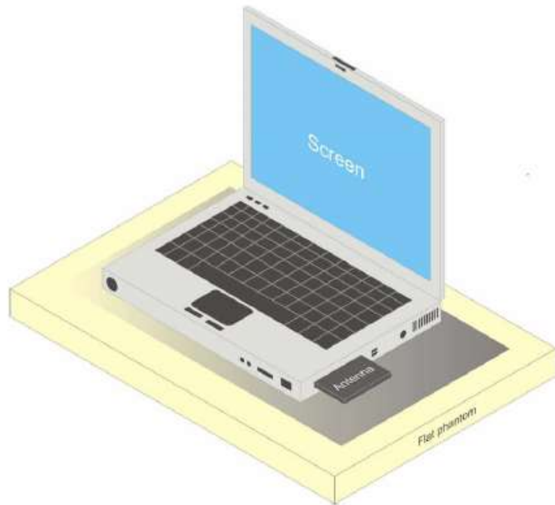
Fig.11.5 Illustration for Body-supported Position
