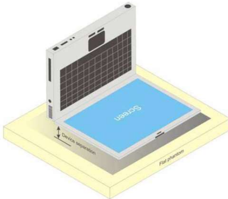
Illustration for Screen antenna EUT test Position
