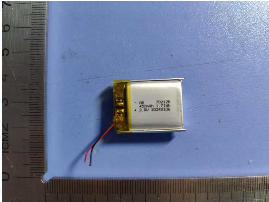
Photo 8 Battery appearance
