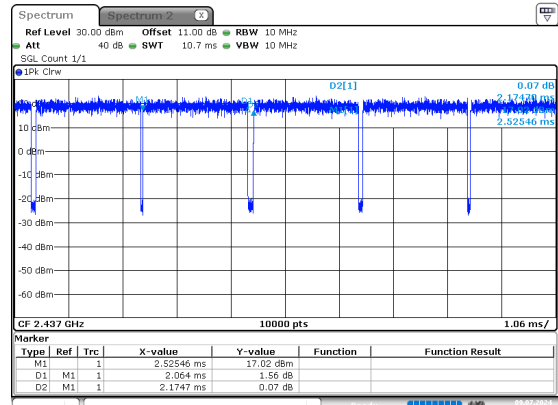
g_2437MHz_Chain 0
