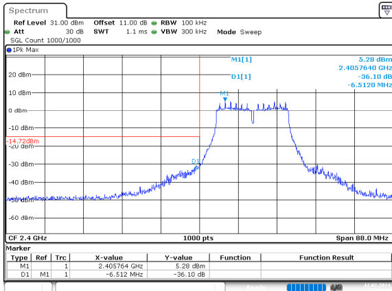
g_2412MHz_Chain 0
