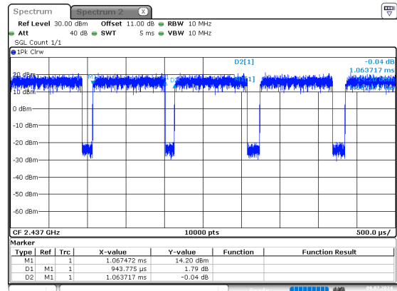
n40_2437MHz_Chain 0
